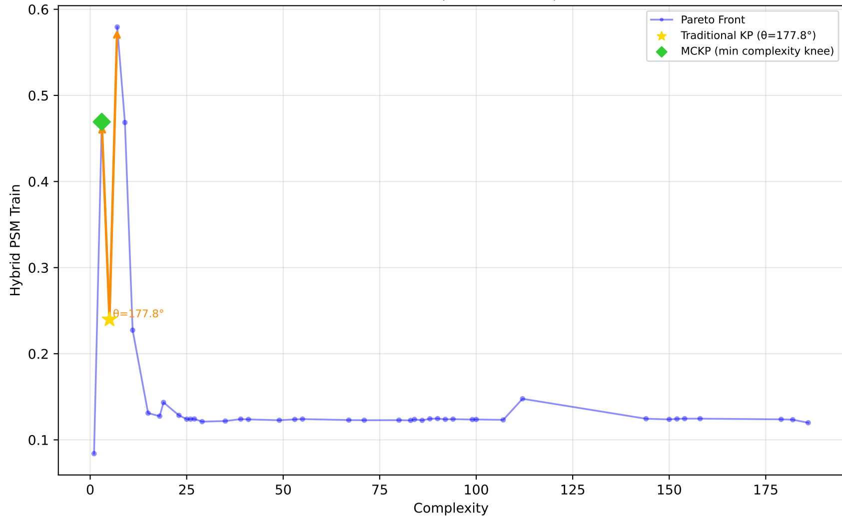
529_pollen - Run 8 - MVP - Hybrid PSM Train \lambda_1=0.90, \lambda_2=0.00, \lambda_3=0.00 | Difficulty: 0.81 | Method: hmr
