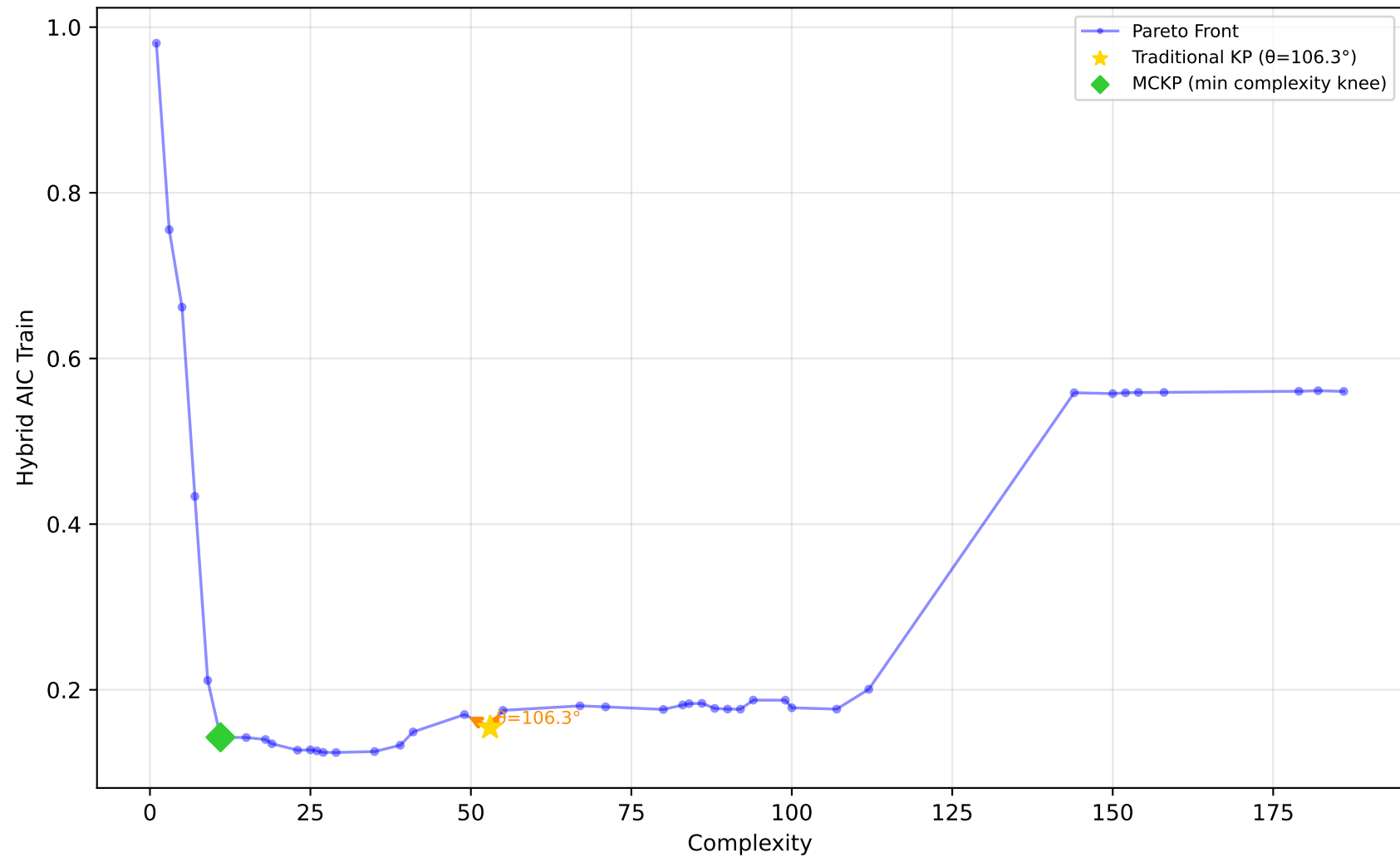
529_pollen - Run 8 - SVP - Hybrid AIC Train \lambda_1=0.60, \lambda_2=0.40, \lambda_3=1.00 | Difficulty: 0.81 | Method: hmr
