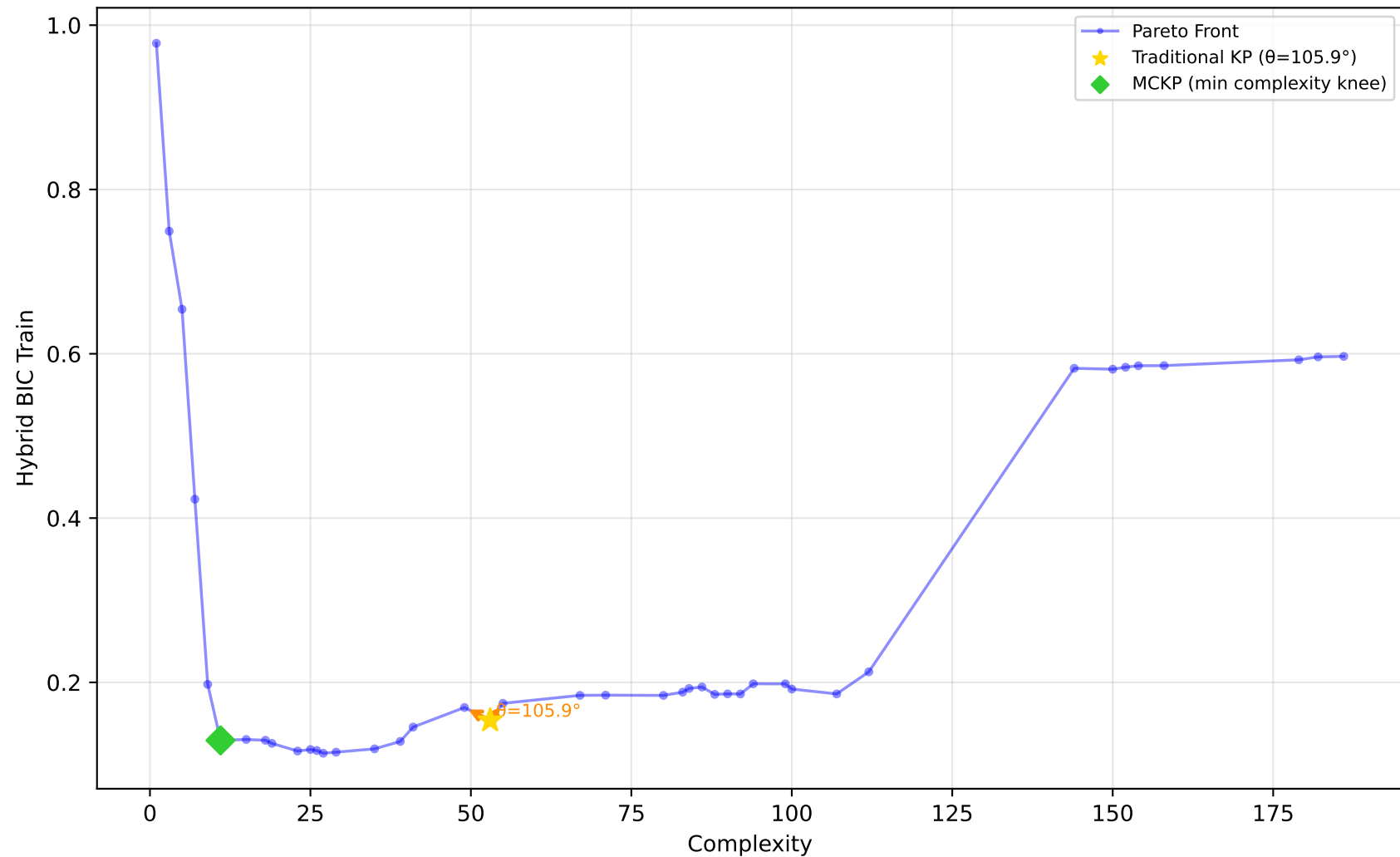
529_pollen - Run 8 - SVP - Hybrid BIC Train \lambda_1=0.60, \lambda_2=0.40, \lambda_3=1.00 | Difficulty: 0.81 | Method: hmr
