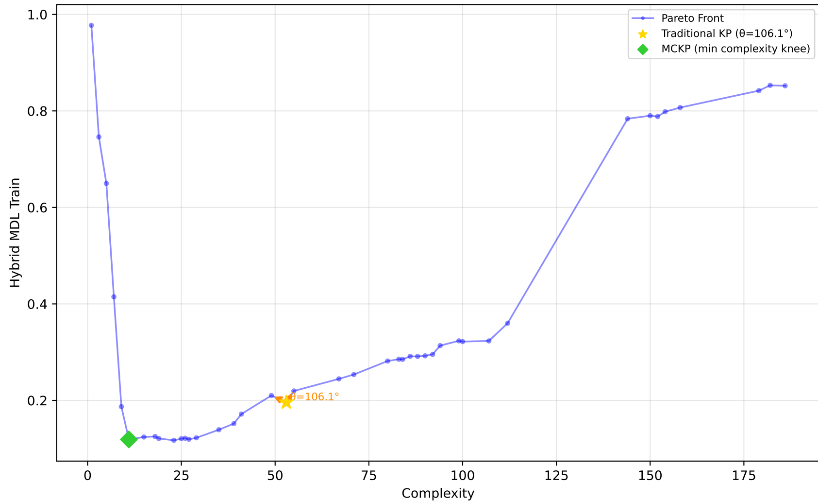
529_pollen - Run 8 - SVP - Hybrid MDL Train \lambda_1=0.60, \lambda_2=0.40, \lambda_3=1.00 | Difficulty: 0.81 | Method: hmr
