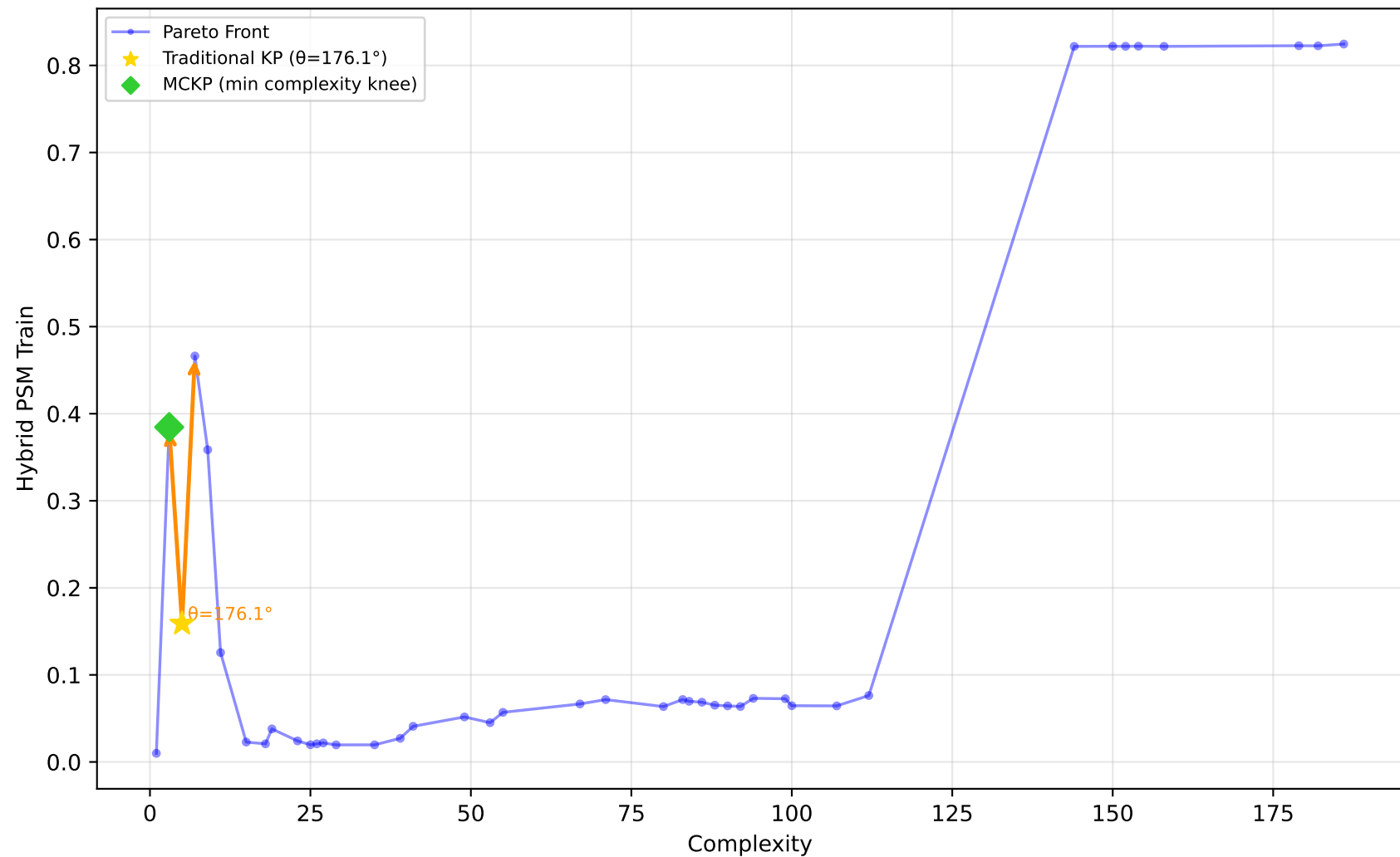
529_pollen - Run 8 - SVP - Hybrid PSM Train \lambda_1=0.10, \lambda_2=0.80, \lambda_3=0.30 | Difficulty: 0.81 | Method: hmr
