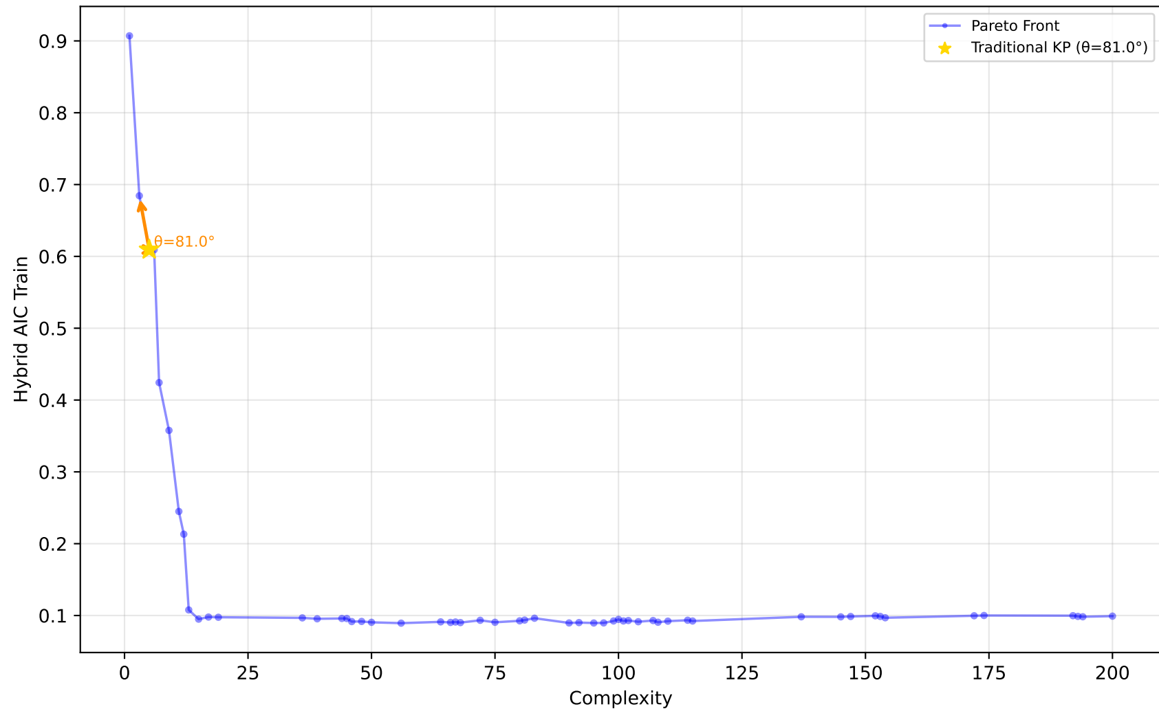
529_pollen - Run 9 - MVP - Hybrid AIC Train \lambda_1=0.00, \lambda_2=1.00, \lambda_3=0.80 | Difficulty: 1.00 | Method: hmr
