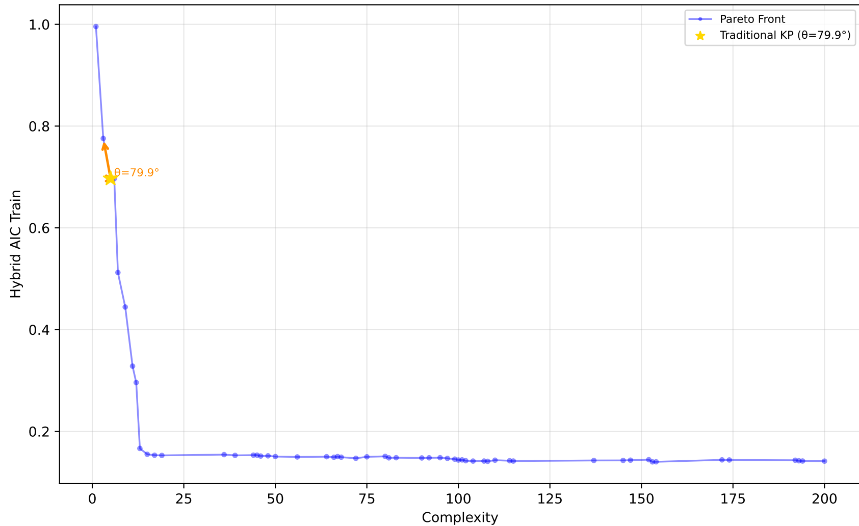
529_pollen - Run 9 - MVP - Hybrid AIC Train \lambda_1=0.90, \lambda_2=0.00, \lambda_3=0.00 | Difficulty: 1.00 | Method: hmr
