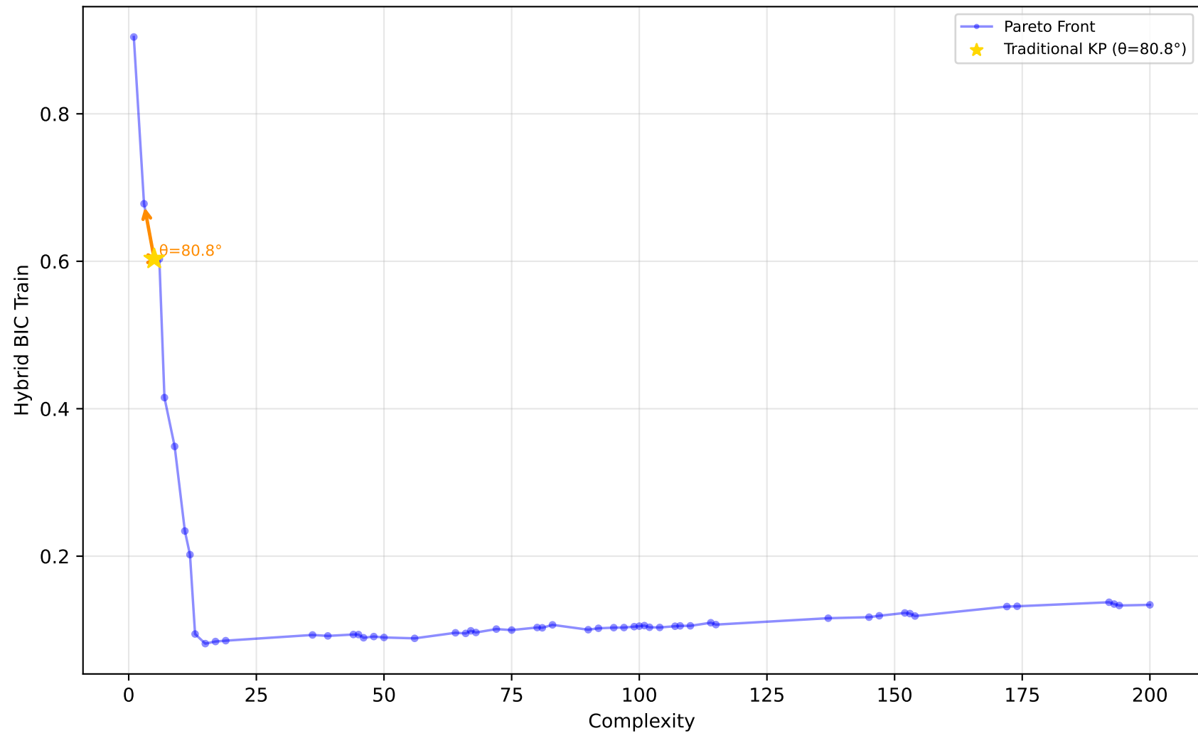
529_pollen - Run 9 - MVP - Hybrid BIC Train \lambda_1=0.00 , \lambda_2=1.00 , \lambda_3=0.80 | Difficulty: 1.00 | Method: hmr
