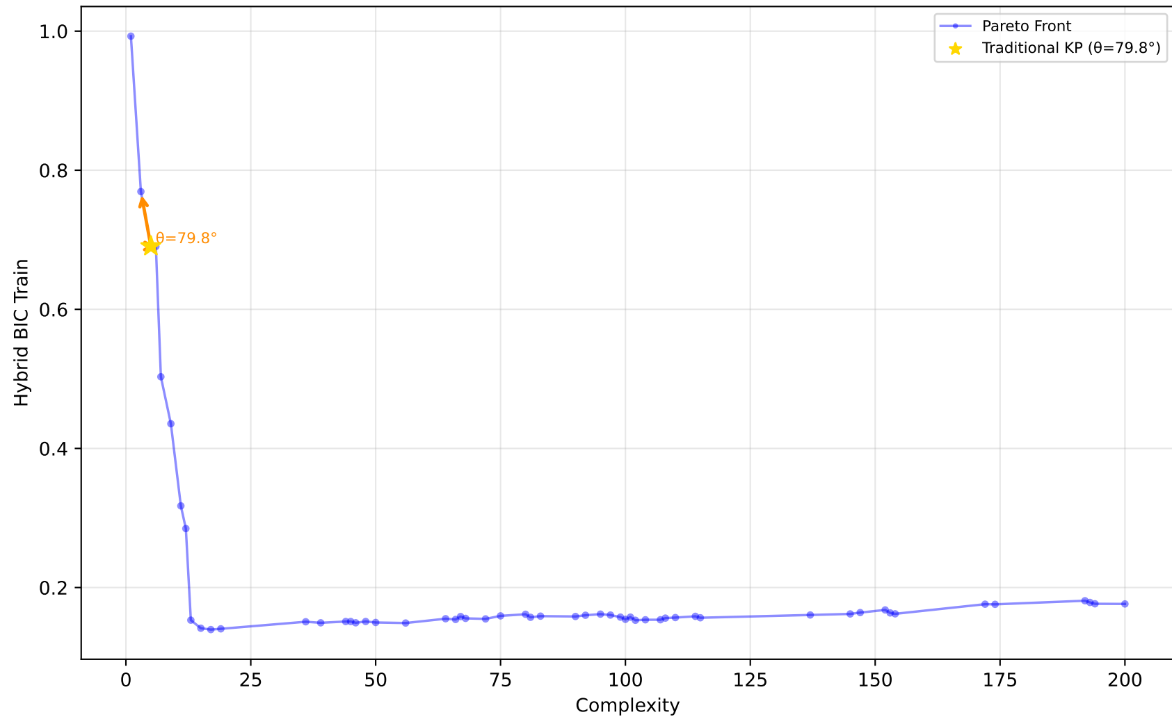
529_pollen - Run 9 - MVP - Hybrid BIC Train \lambda_1=0.90, \lambda_2=0.00, \lambda_3=0.00 | Difficulty: 1.00 | Method: hmr
