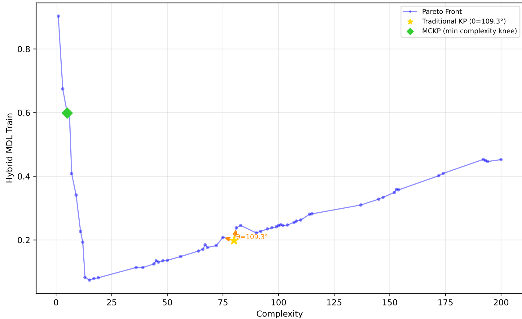
529_pollen - Run 9 - MVP - Hybrid MDL Train \lambda_1=0.00, \lambda_2=1.00, \lambda_3=0.80 | Difficulty: 1.00 | Method: hmr
