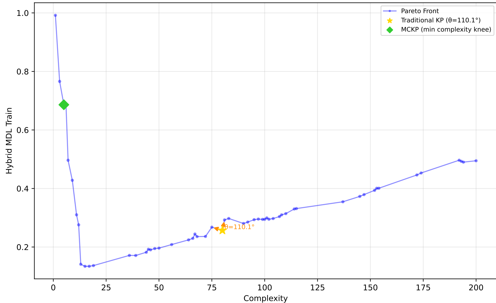
529_pollen - Run 9 - MVP - Hybrid MDL Train \lambda_1=0.90, \lambda_2=0.00, \lambda_3=0.00 | Difficulty: 1.00 | Method: hmr
