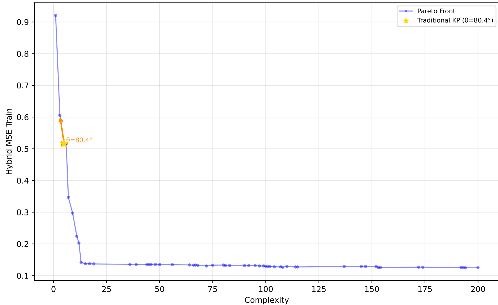
529_pollen - Run 9 - MVP - Hybrid MSE Train \lambda_1=0.90, \lambda_2=0.00, \lambda_3=0.00 | Difficulty: 1.00 | Method: hmr
