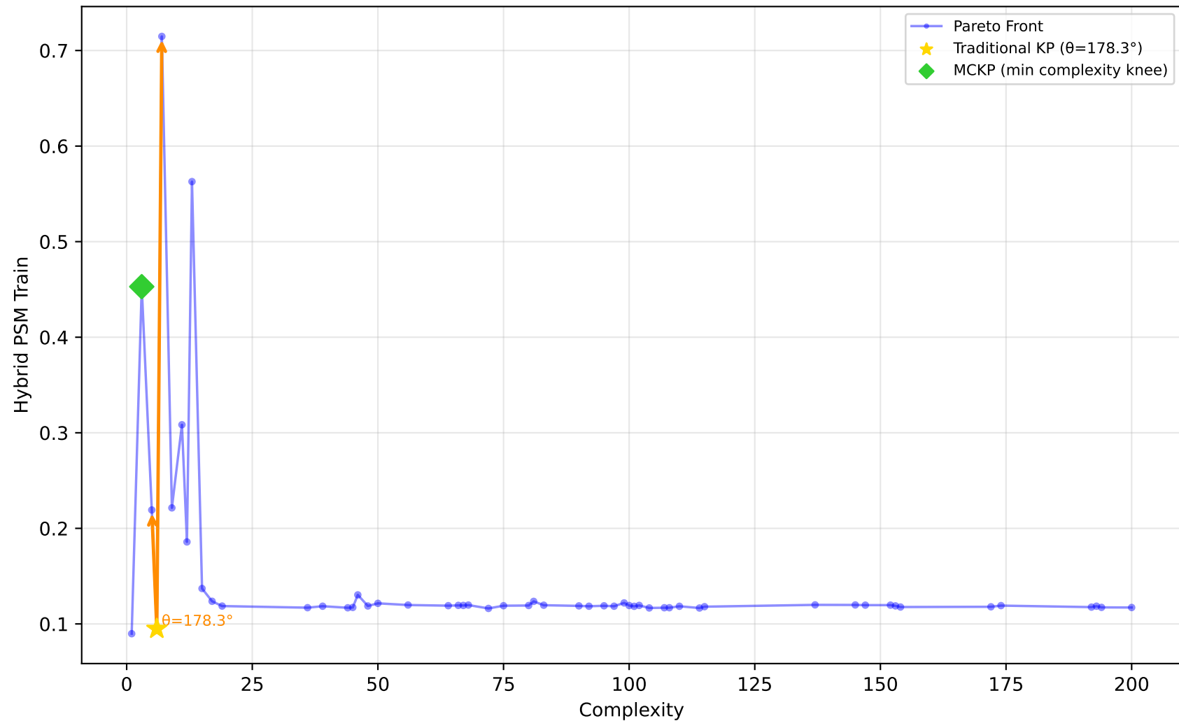
529_pollen - Run 9 - MVP - Hybrid PSM Train \lambda_1=0.90, \lambda_2=0.00, \lambda_3=0.00 | Difficulty: 1.00 | Method: hmr
