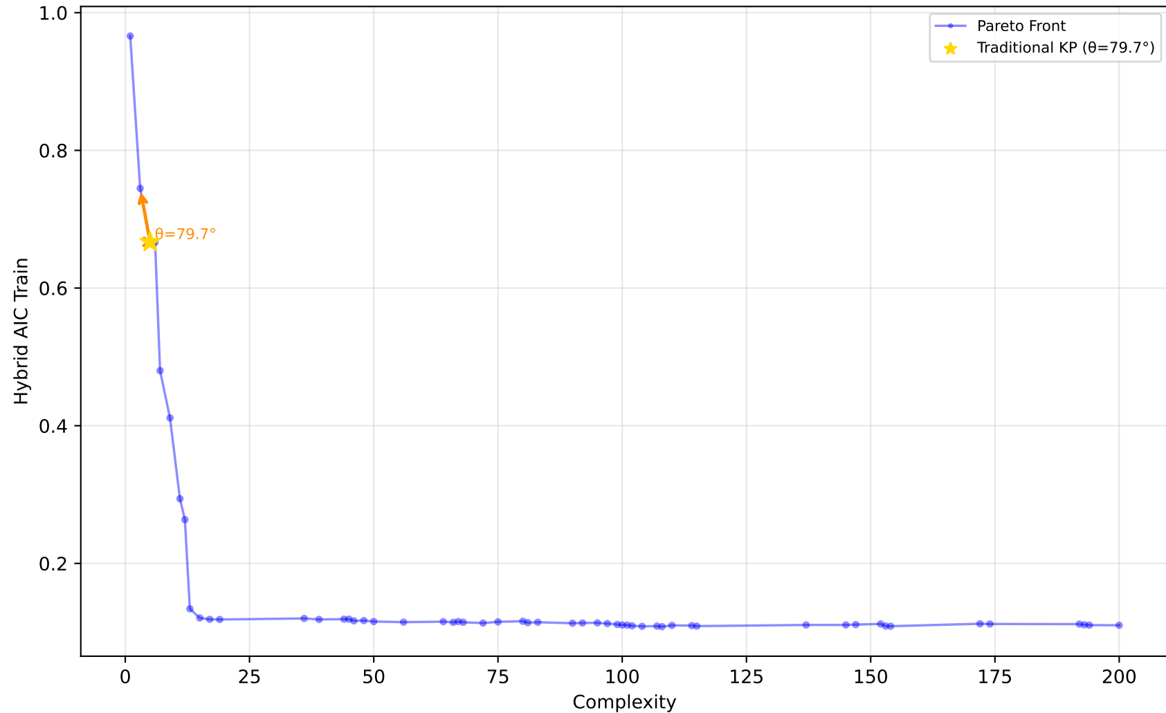
529_pollen - Run 9 - SVP - Hybrid AIC Train \lambda_1=0.60, \lambda_2=0.40, \lambda_3=1.00 | Difficulty: 1.00 | Method: hmr
