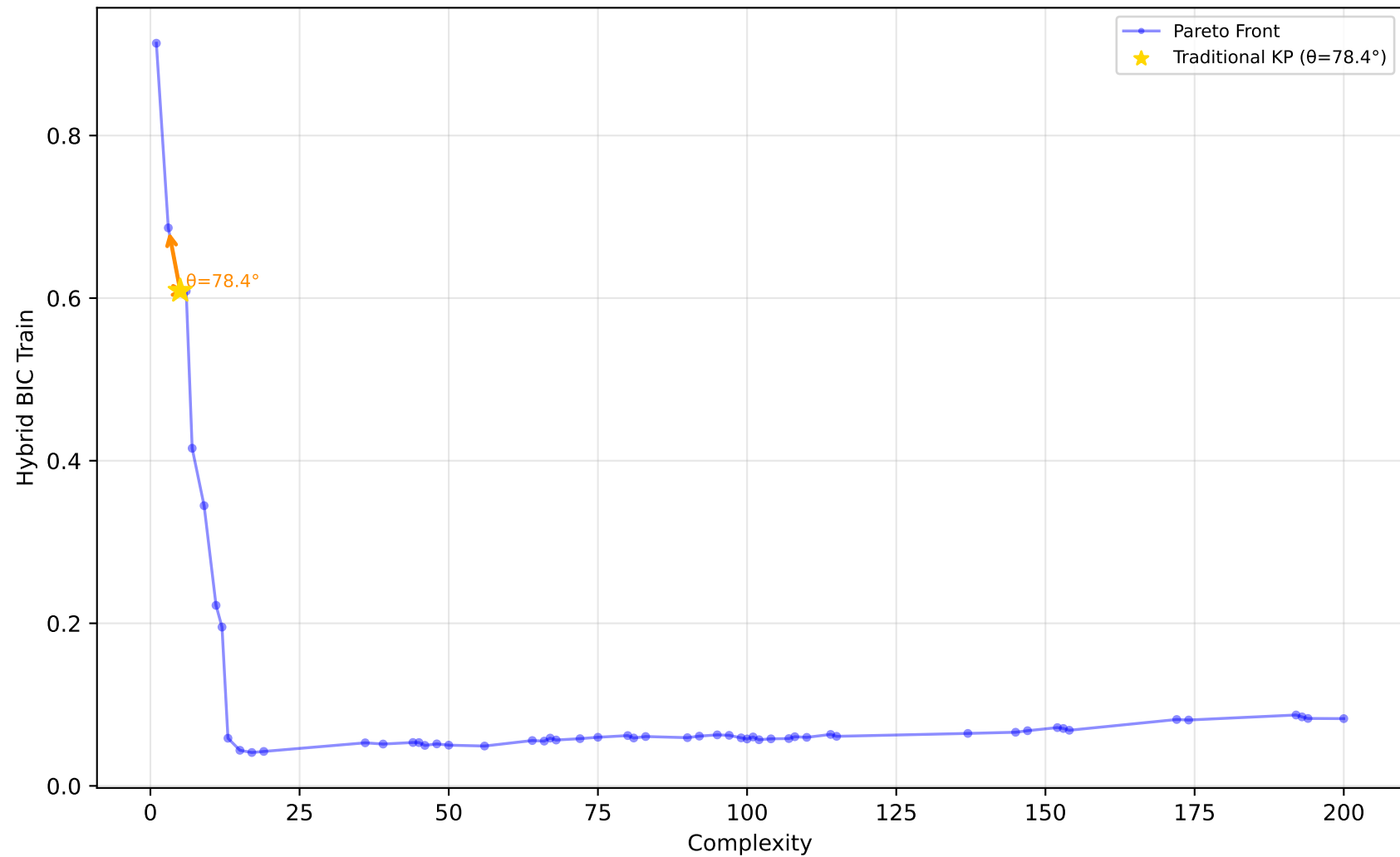
529_pollen - Run 9 - SVP - Hybrid BIC Train \lambda_1=0.10, \lambda_2=0.80, \lambda_3=0.30 | Difficulty: 1.00 | Method: hmr
