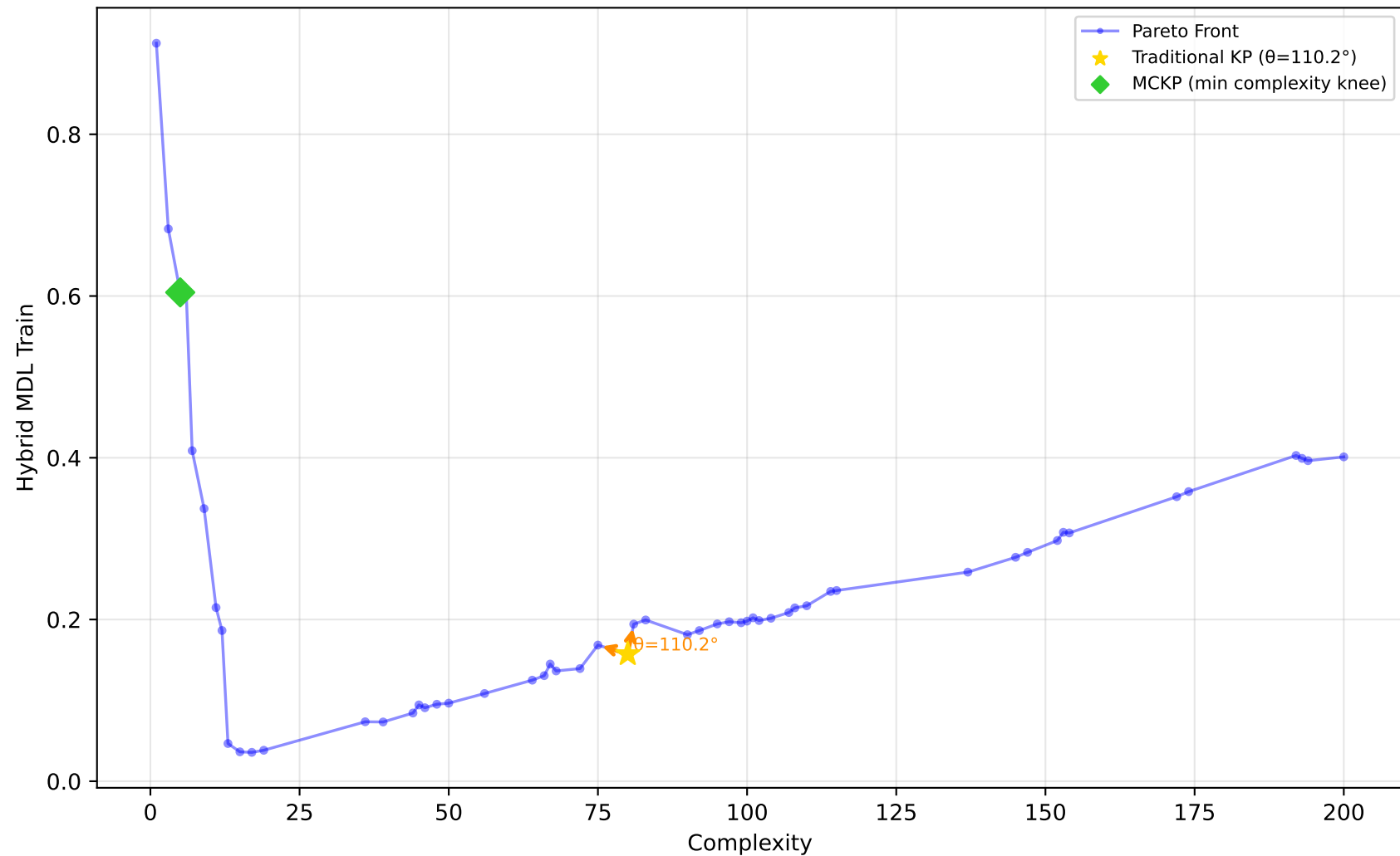
529_pollen - Run 9 - SVP - Hybrid MDL Train \lambda_1=0.10, \lambda_2=0.80, \lambda_3=0.30 | Difficulty: 1.00 | Method: hmr
