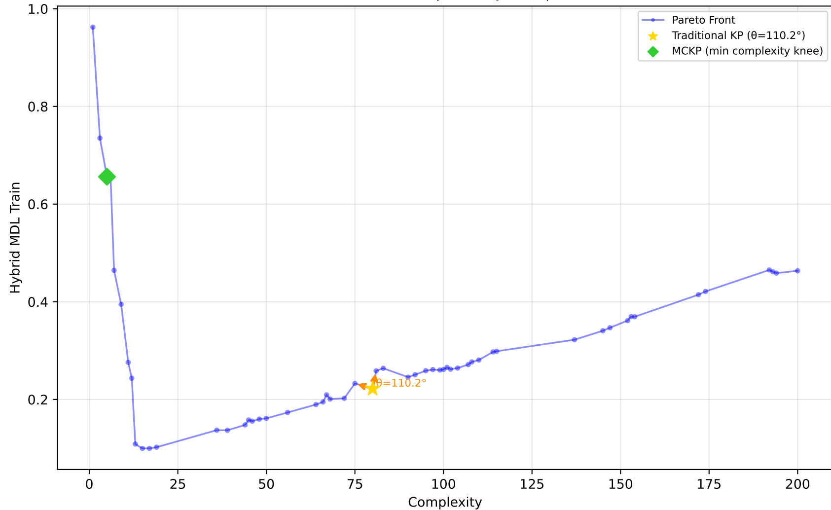
529_pollen - Run 9 - SVP - Hybrid MDL Train \lambda_1=0.60, \lambda_2=0.40, \lambda_3=1.00 | Difficulty: 1.00 | Method: hmr
