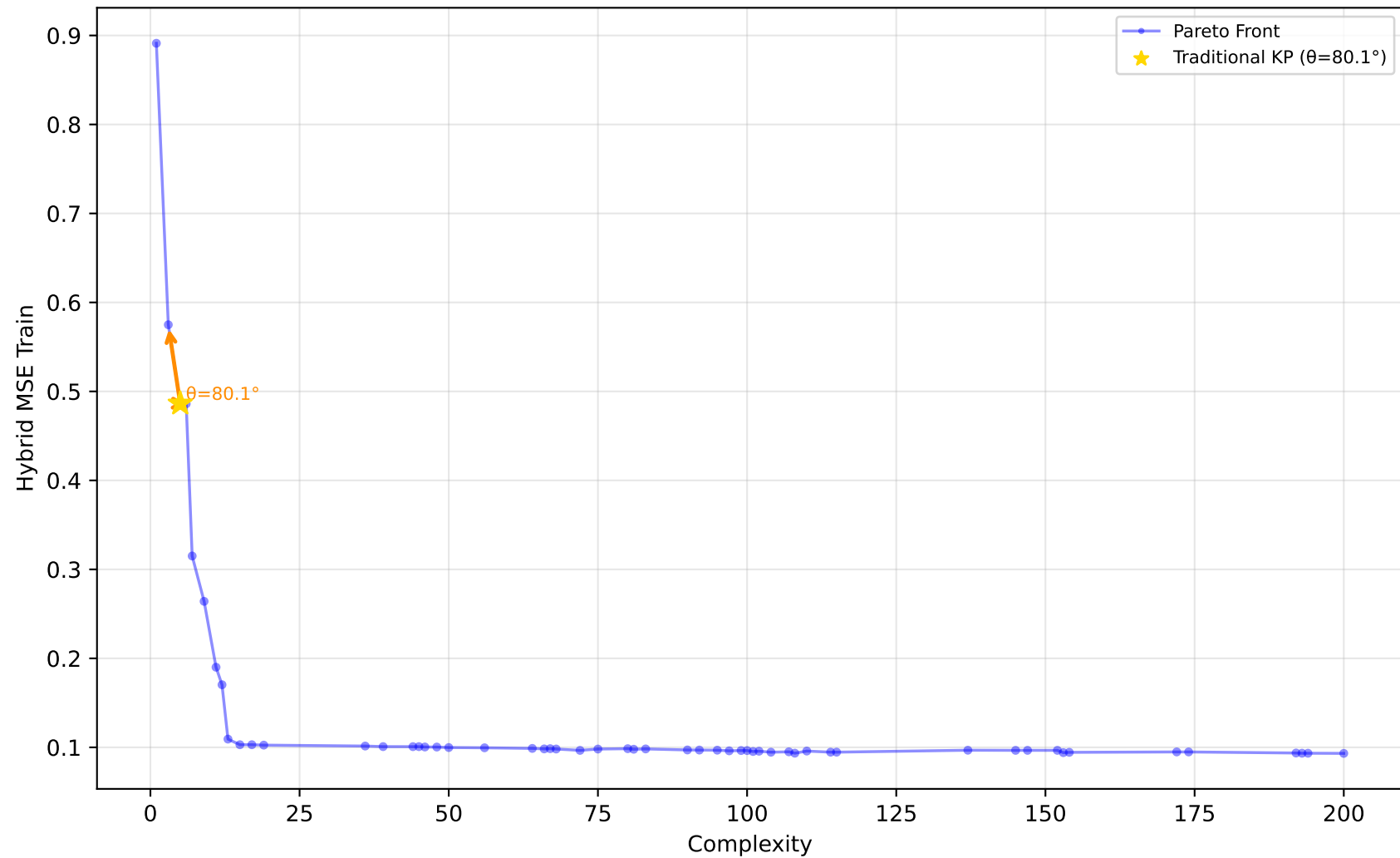
529_pollen - Run 9 - SVP - Hybrid MSE Train \lambda_1=0.60, \lambda_2=0.40, \lambda_3=1.00 | Difficulty: 1.00 | Method: hmr
