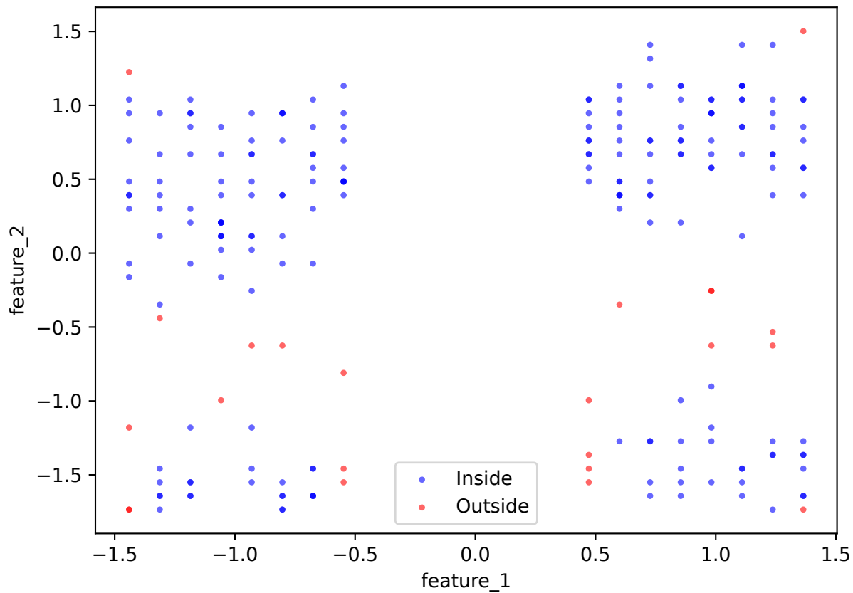
Plot with Bandwidth: 0.41
