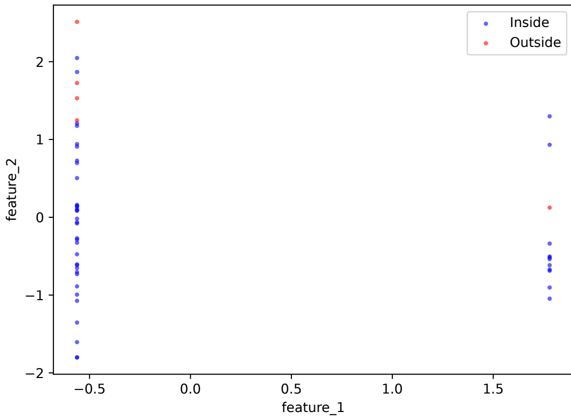
Plot with Bandwidth: 0.10
