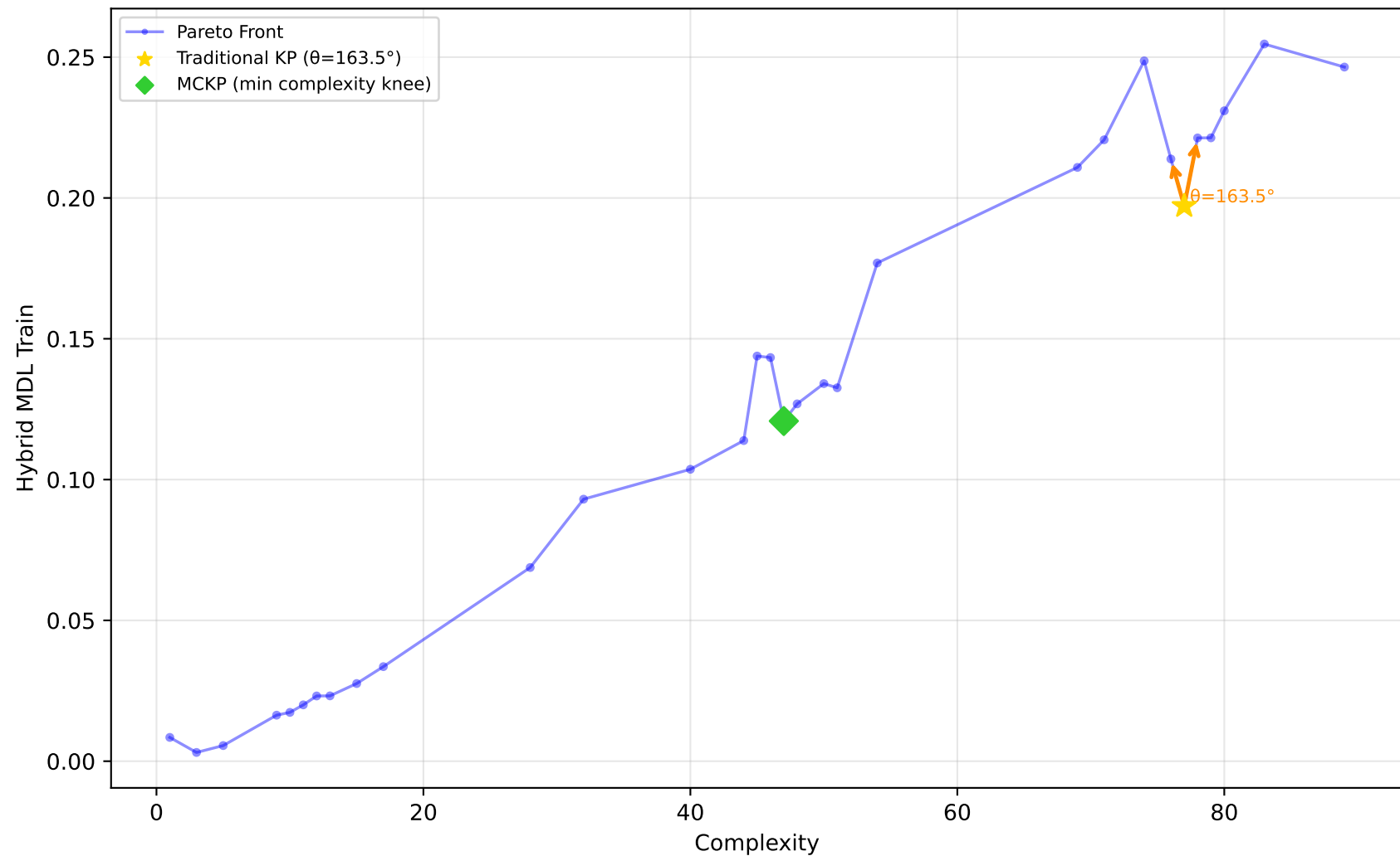
678_visualizing_environmental - Run 10 - MVP - Hybrid MDL Train \lambda_1=0.00, \lambda_2=0.00, \lambda_3=0.10 | Difficulty: 1.00 | Method: hmr
