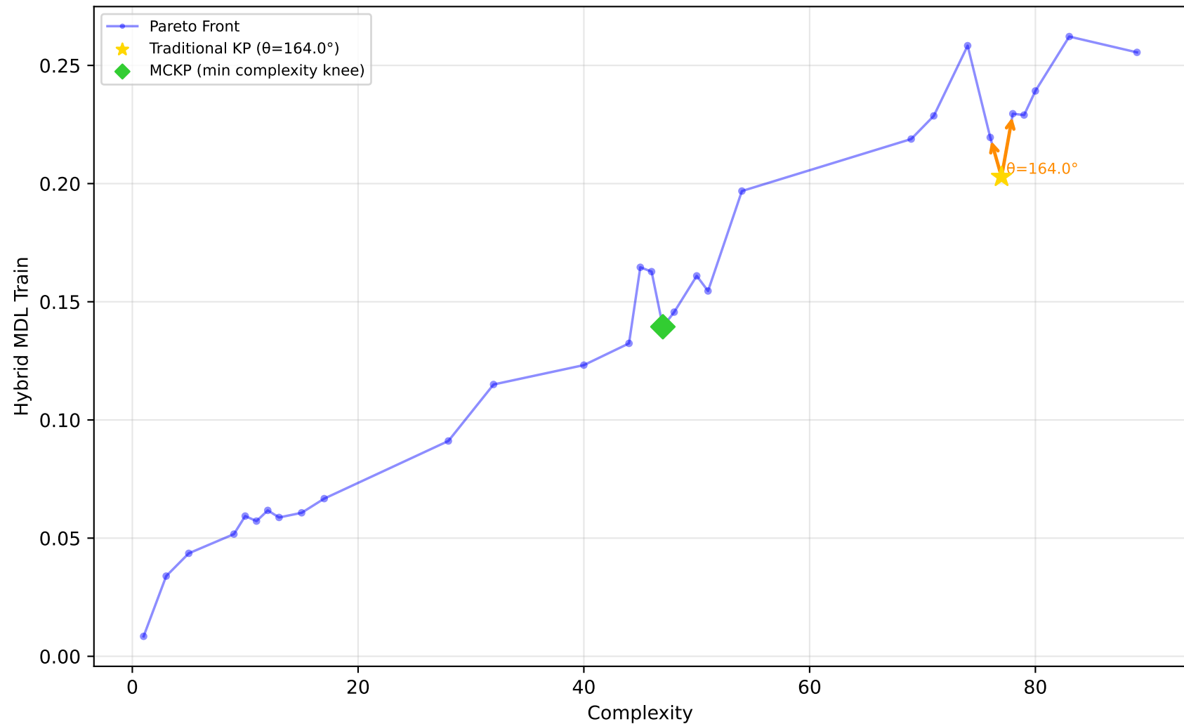
678_visualizing_environmental - Run 10 - MVP - Hybrid MDL Train \lambda_1=0.40 , \lambda_2=0.00 , \lambda_3=0.00 | Difficulty: 1.00 | Method: hmr
