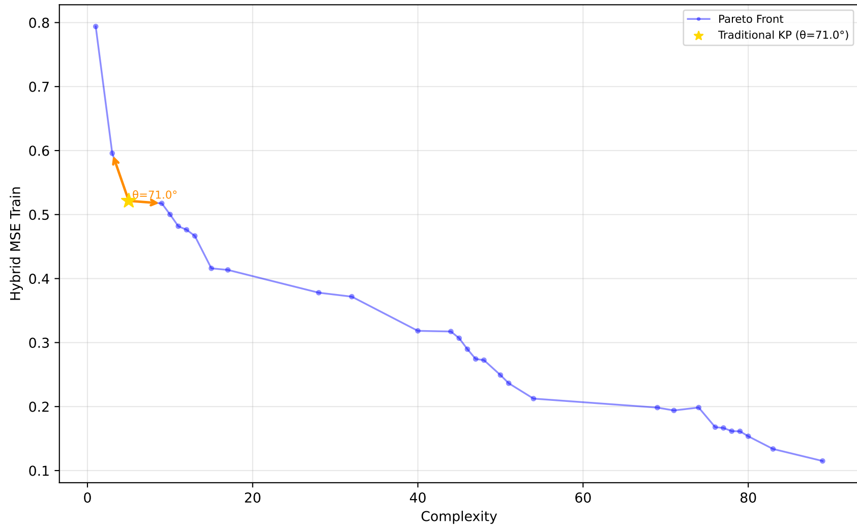
678_visualizing_environmental - Run 10 - MVP - Hybrid MSE Train \lambda_1=0.00, \lambda_2=0.00, \lambda_3=0.10 | Difficulty: 1.00 | Method: hmr
