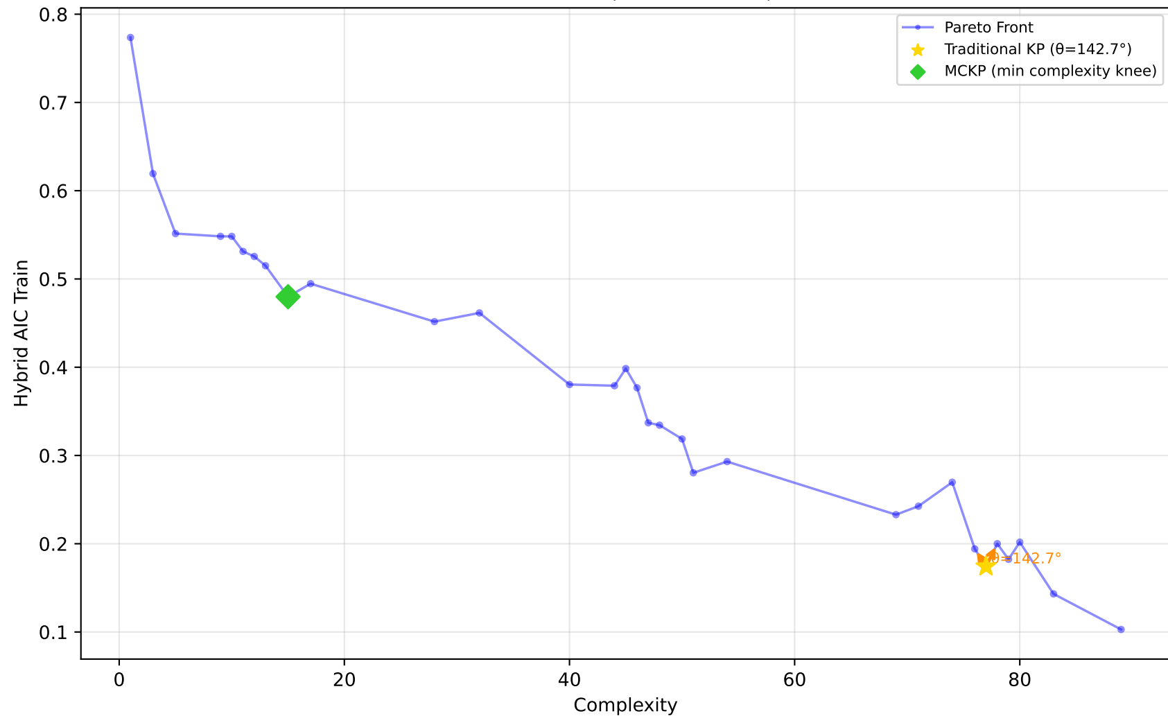
678_visualizing_environmental - Run 10 - SVP - Hybrid AIC Train \lambda_1=0.00, \lambda_2=0.10, \lambda_3=0.20 | Difficulty: 1.00 | Method: hmr
