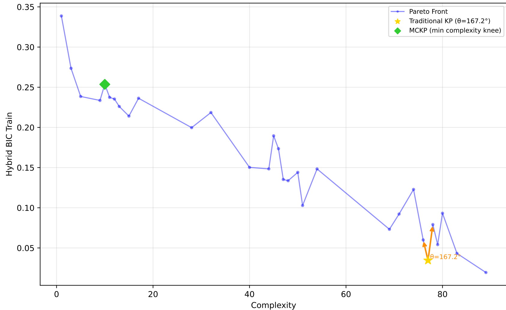
678_visualizing_environmental - Run 10 - SVP - Hybrid BIC Train \lambda_1=0.40, \lambda_2=0.00, \lambda_3=0.00 | Difficulty: 1.00 | Method: hmr
