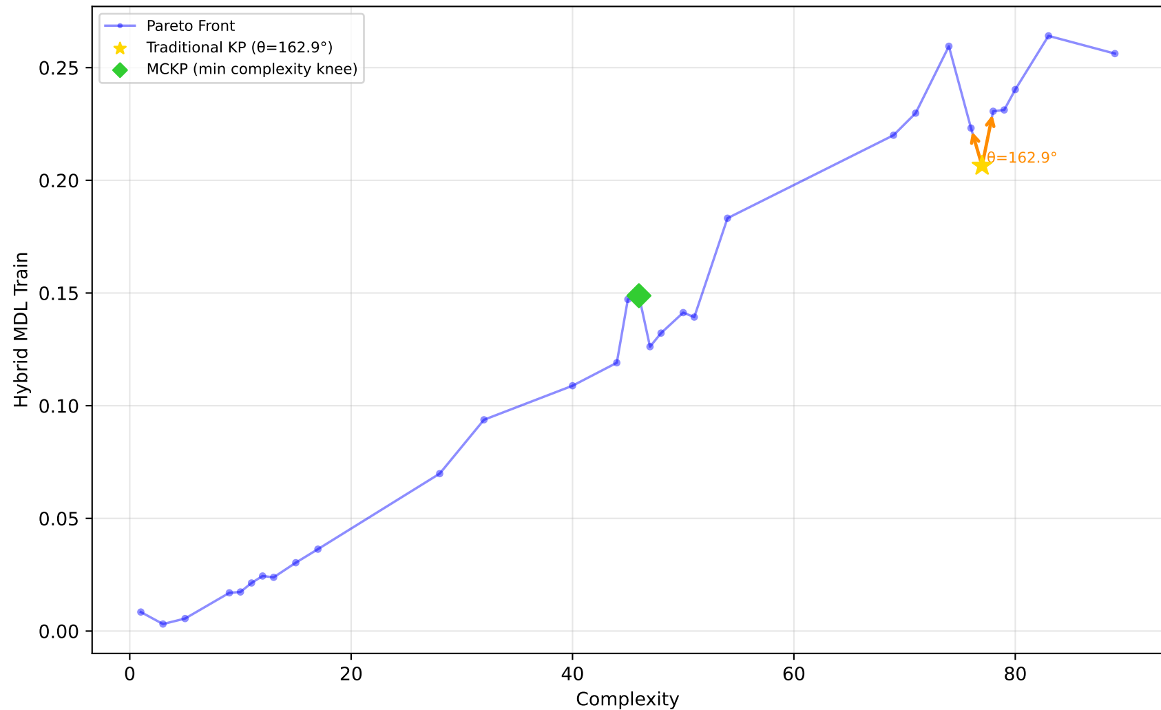
678_visualizing_environmental - Run 10 - SVP - Hybrid MDL Train \lambda_1=0.00, \lambda_2=0.10, \lambda_3=0.20 | Difficulty: 1.00 | Method: hmr
