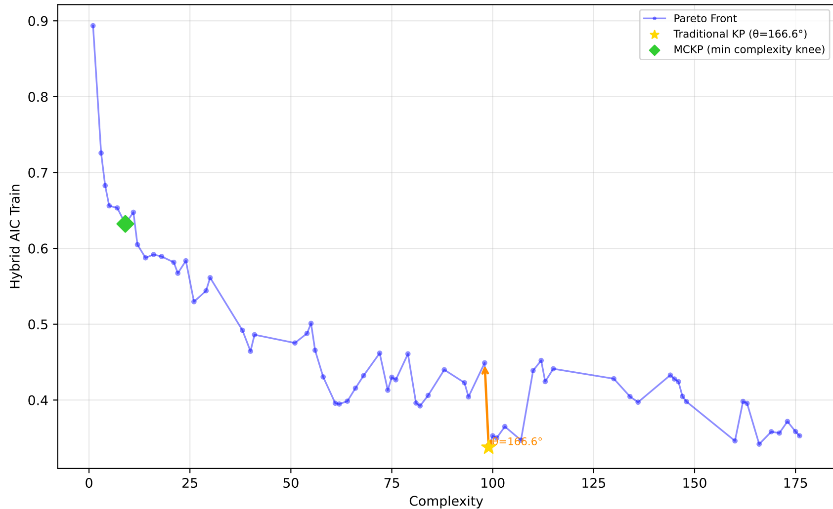
678_visualizing_environmental - Run 12 - MVP - Hybrid AIC Train \lambda_1=0.00, \lambda_2=0.00, \lambda_3=0.10 | Difficulty: 1.00 | Method: hmr
