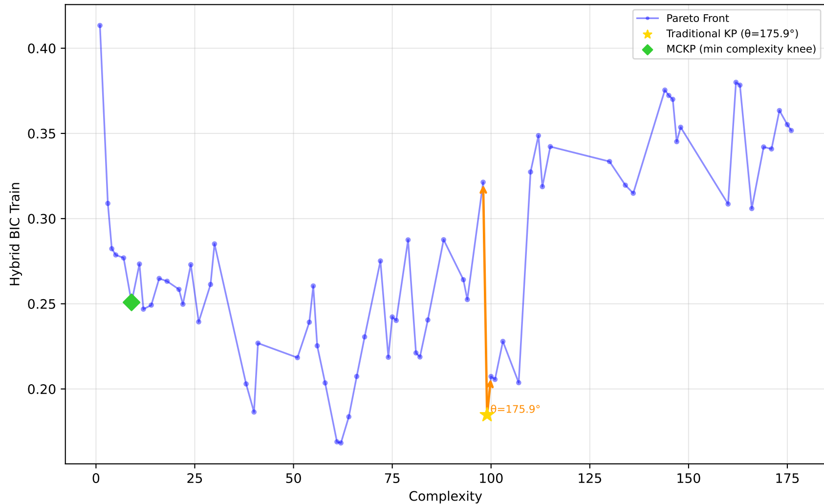
678_visualizing_environmental - Run 12 - MVP - Hybrid BIC Train \lambda_1=0.00, \lambda_2=0.00, \lambda_3=0.10 | Difficulty: 1.00 | Method: hmr
