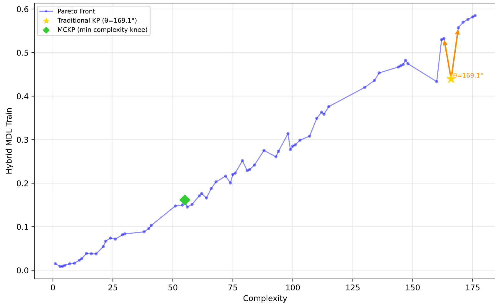
678_visualizing_environmental - Run 12 - MVP - Hybrid MDL Train \lambda_1=0.00, \lambda_2=0.00, \lambda_3=0.10 | Difficulty: 1.00 | Method: hmr
