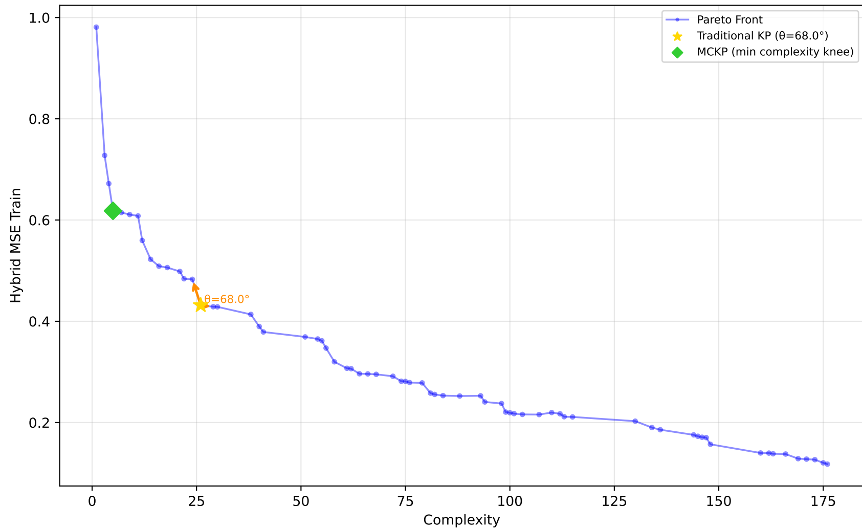
678_visualizing_environmental - Run 12 - MVP - Hybrid MSE Train \lambda_1=0.00, \lambda_2=0.00, \lambda_3=0.10 | Difficulty: 1.00 | Method: hmr
