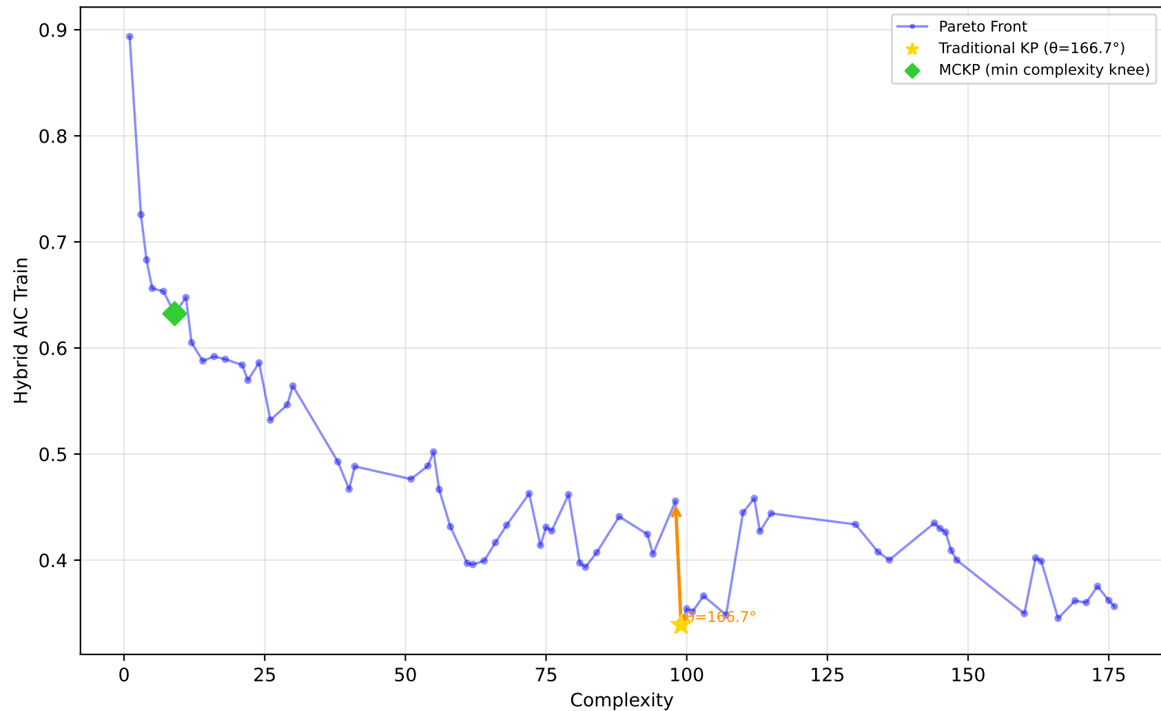
678_visualizing_environmental - Run 12 - SVP - Hybrid AIC Train \lambda_1=0.00, \lambda_2=0.10, \lambda_3=0.20 | Difficulty: 1.00 | Method: hmr
