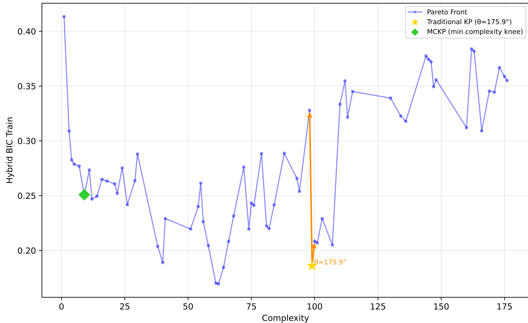
678_visualizing_environmental - Run 12 - SVP - Hybrid BIC Train \lambda_1=0.00, \lambda_2=0.10, \lambda_3=0.20 | Difficulty: 1.00 | Method: hmr
