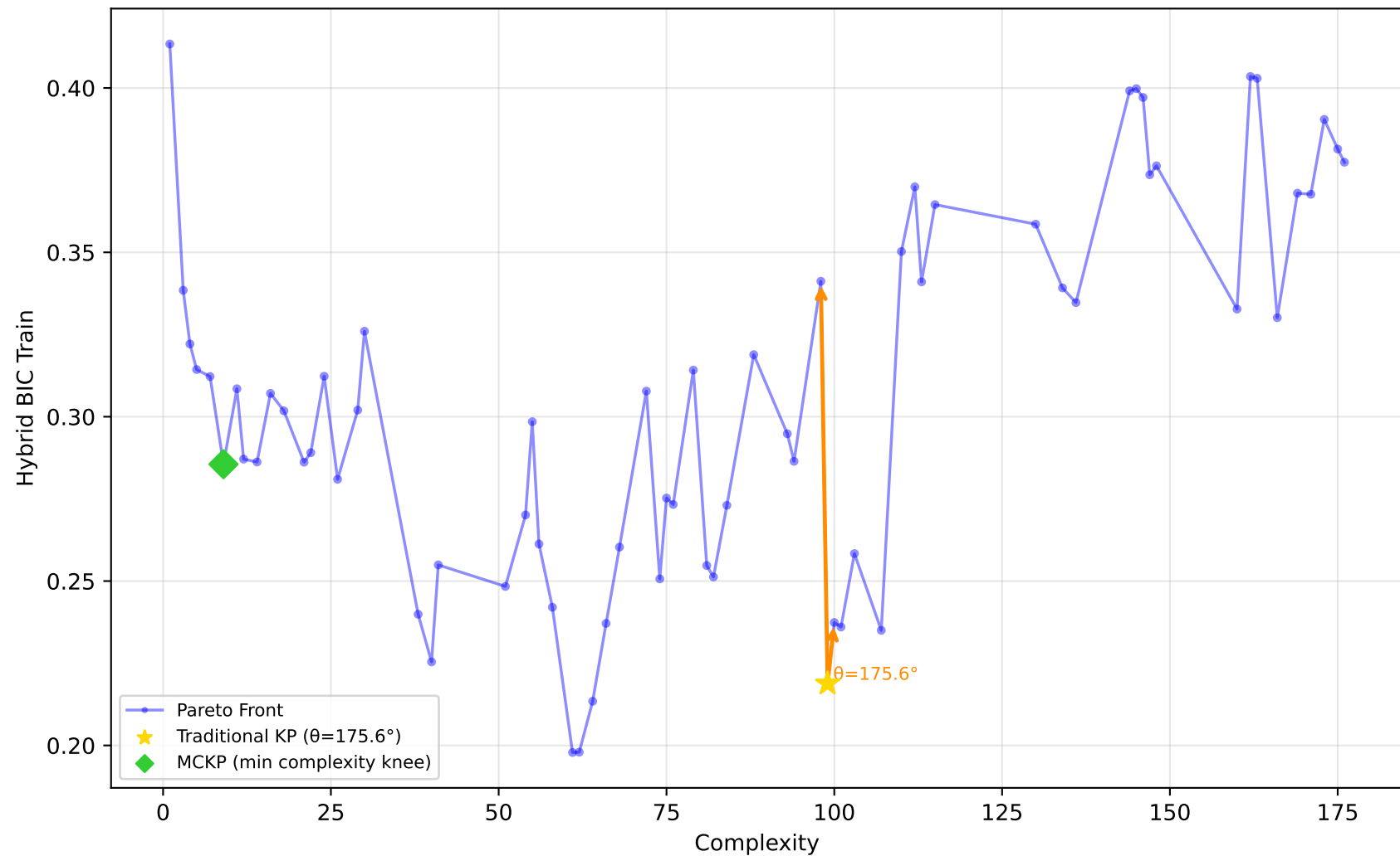
678_visualizing_environmental - Run 12 - SVP - Hybrid BIC Train \lambda_1=0.40 , \lambda_2=0.00 , \lambda_3=0.00 | Difficulty: 1.00 | Method: hmr
