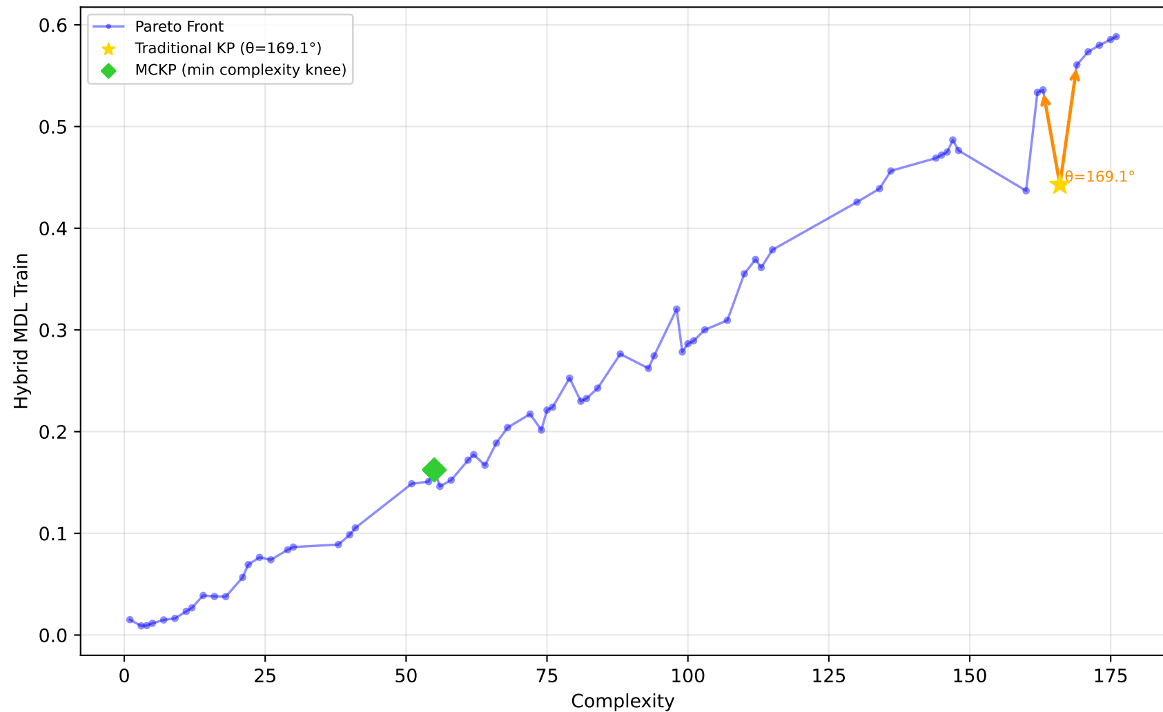
678_visualizing_environmental - Run 12 - SVP - Hybrid MDL Train \lambda_1=0.00, \lambda_2=0.10, \lambda_3=0.20 | Difficulty: 1.00 | Method: hmr
