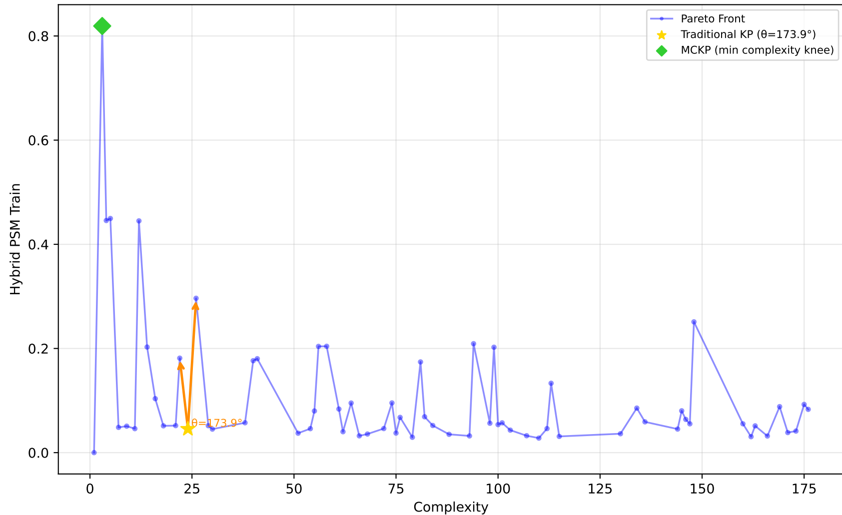
678_visualizing_environmental - Run 12 - SVP - Hybrid PSM Train \lambda_1=0.40, \lambda_2=0.00, \lambda_3=0.00 | Difficulty: 1.00 | Method: hmr
