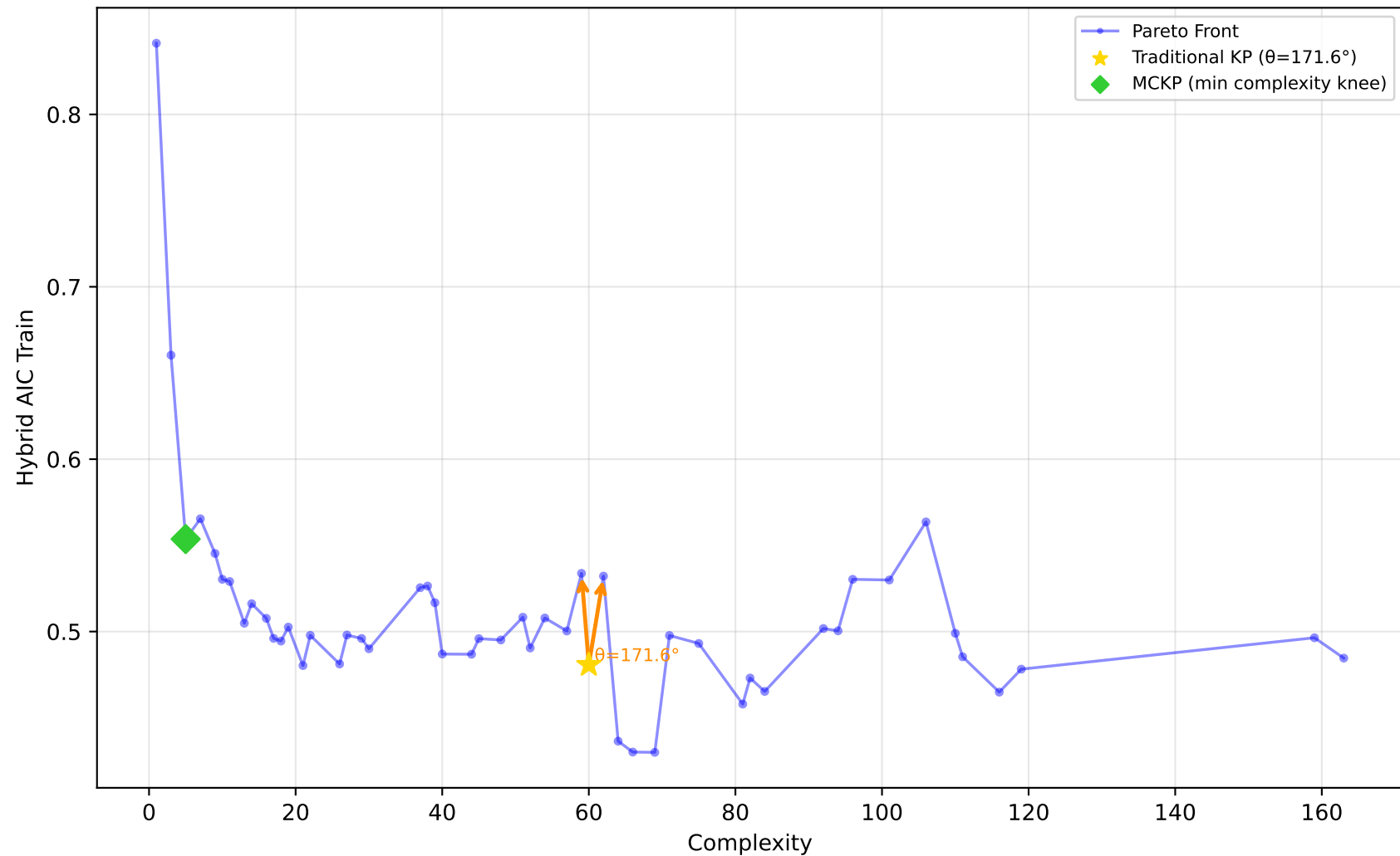
678_visualizing_environmental - Run 13 - MVP - Hybrid AIC Train \lambda_1=0.00, \lambda_2=0.00, \lambda_3=0.10 | Difficulty: 0.11 | Method: mckp
