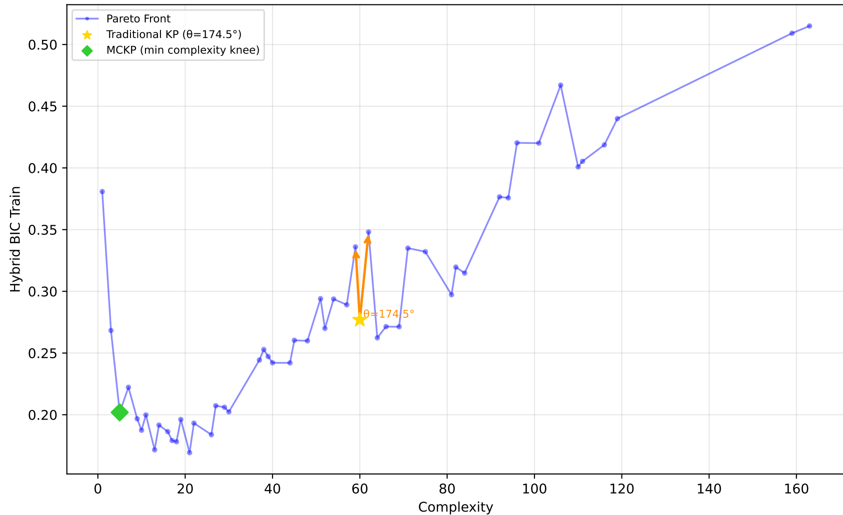
678_visualizing_environmental - Run 13 - MVP - Hybrid BIC Train \lambda_1=0.00, \lambda_2=0.00, \lambda_3=0.10 | Difficulty: 0.11 | Method: mckp
