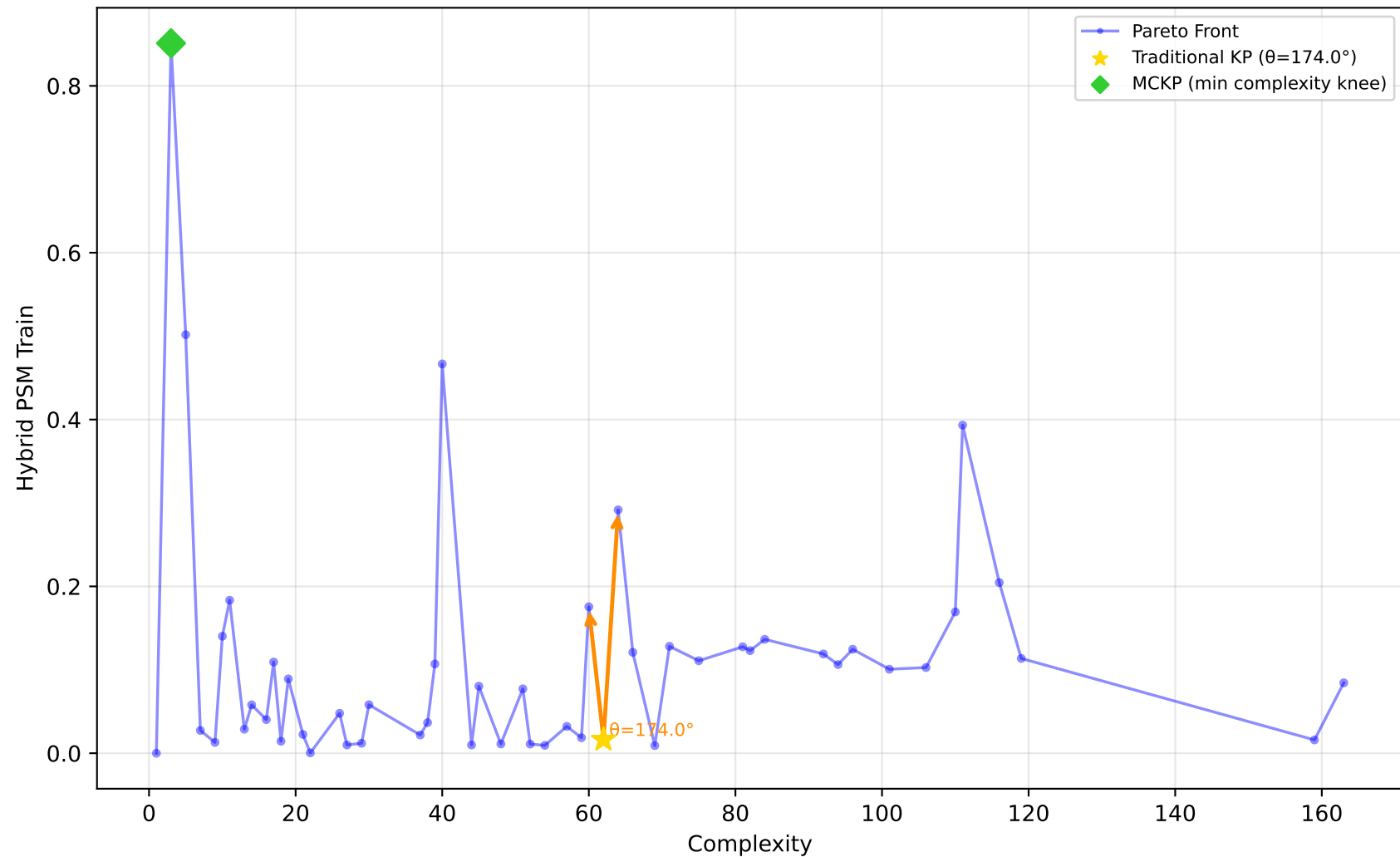
678_visualizing_environmental - Run 13 - MVP - Hybrid PSM Train \lambda_1=0.00, \lambda_2=0.00, \lambda_3=0.10 | Difficulty: 0.11 | Method: mckp
