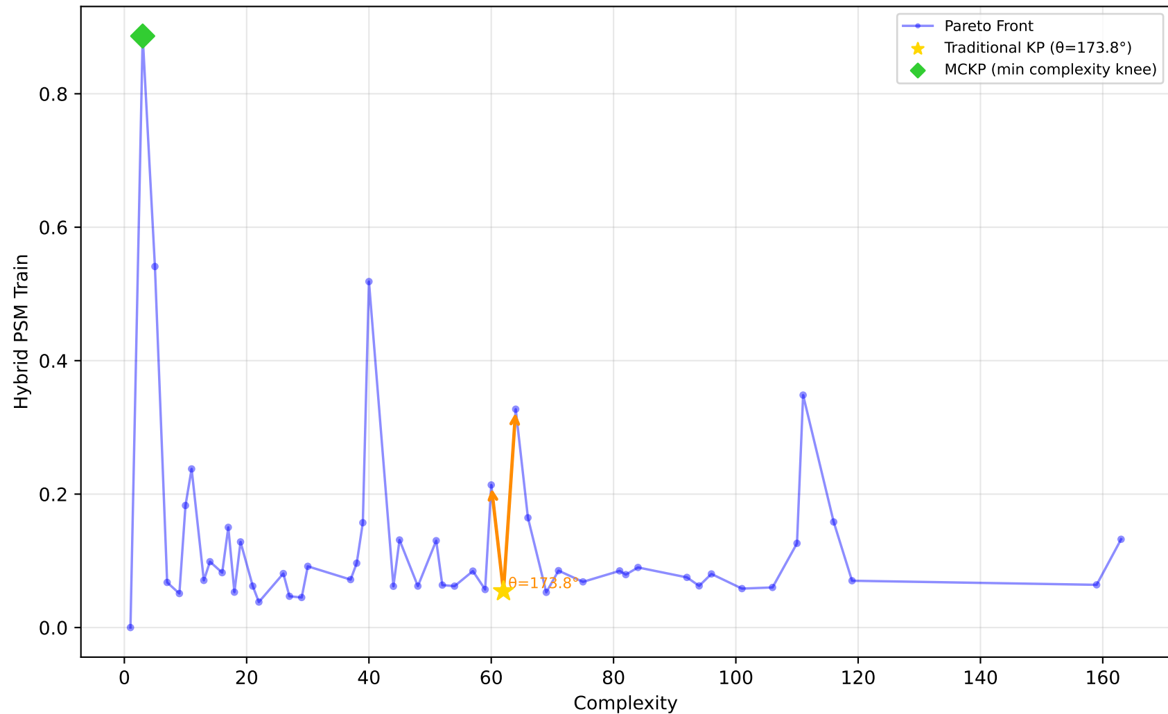
678_visualizing_environmental - Run 13 - MVP - Hybrid PSM Train \lambda_1=0.40, \lambda_2=0.00, \lambda_3=0.00 | Difficulty: 0.11 | Method: mckp
