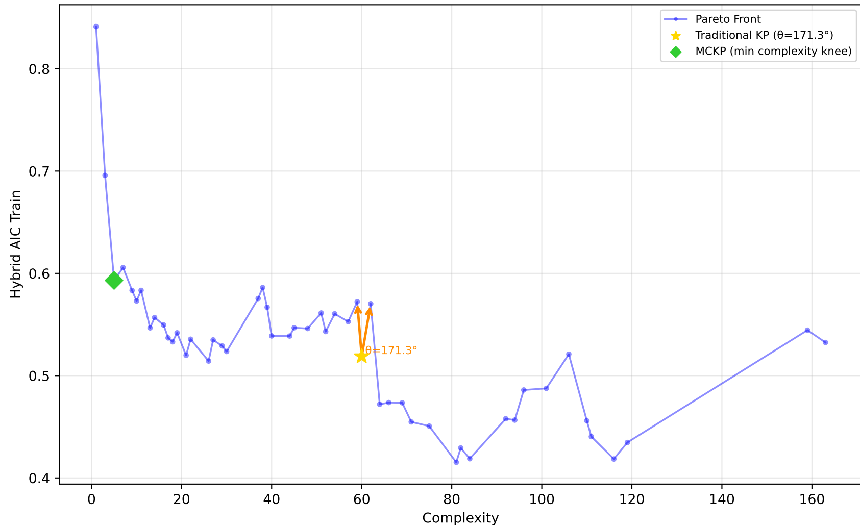
678_visualizing_environmental - Run 13 - SVP - Hybrid AIC Train \lambda_1=0.40, \lambda_2=0.00, \lambda_3=0.00 | Difficulty: 0.11 | Method: mckp
