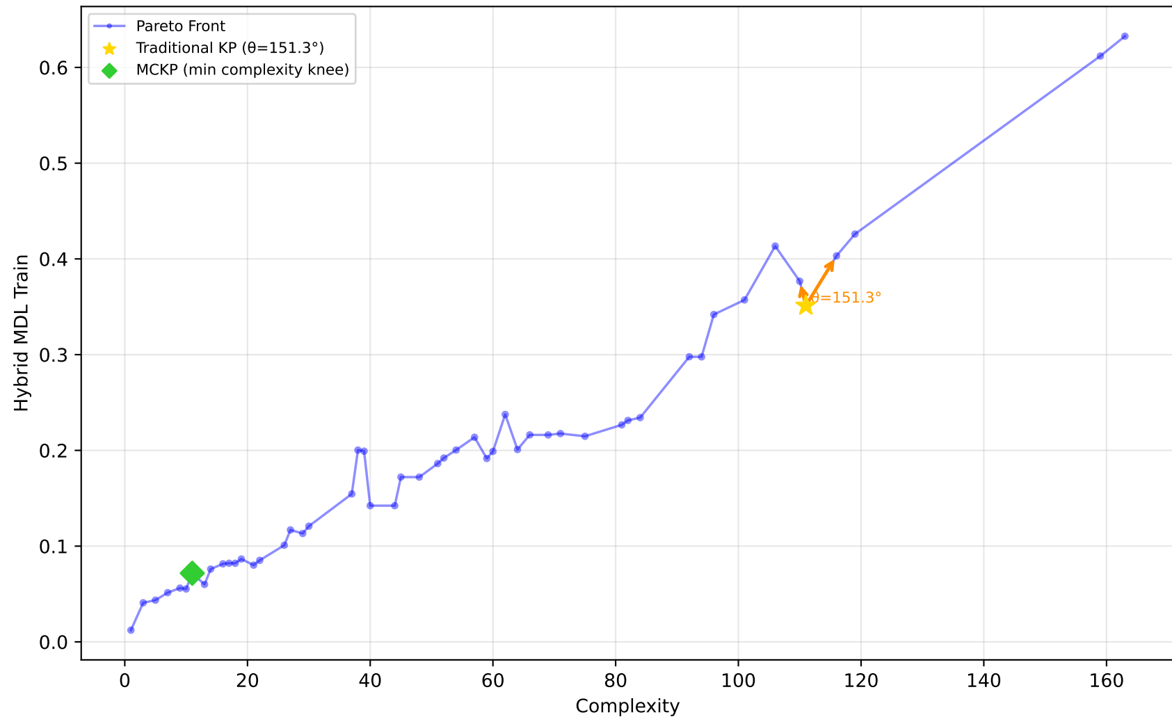
678_visualizing_environmental - Run 13 - SVP - Hybrid MDL Train \lambda_1=0.40, \lambda_2=0.00, \lambda_3=0.00 | Difficulty: 0.11 | Method: mckp
