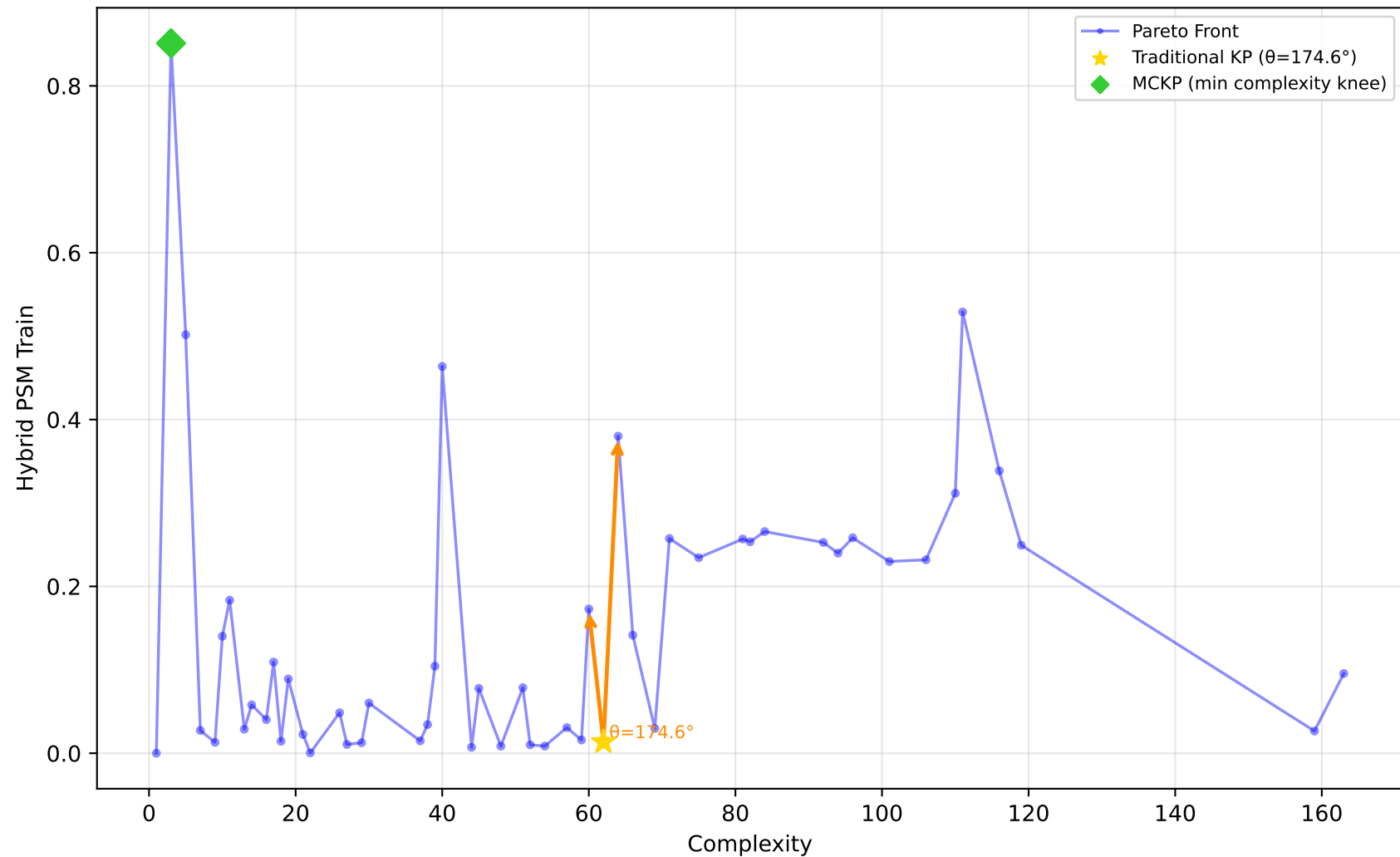
678_visualizing_environmental - Run 13 - SVP - Hybrid PSM Train \lambda_1=0.00, \lambda_2=0.10, \lambda_3=0.20 | Difficulty: 0.11 | Method: mckp
