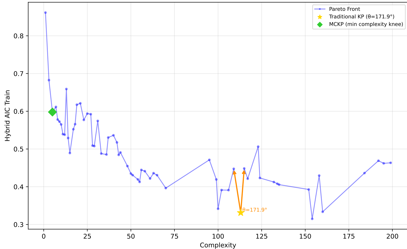
678_visualizing_environmental - Run 14 - MVP - Hybrid AIC Train \lambda_1=0.00, \lambda_2=0.00, \lambda_3=0.10 | Difficulty: 0.25 | Method: mckp
