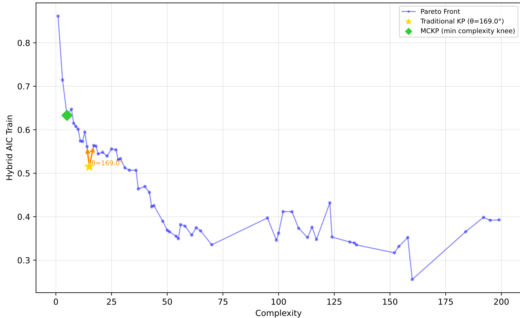
678_visualizing_environmental - Run 14 - MVP - Hybrid AIC Train \lambda_1=0.40, \lambda_2=0.00, \lambda_3=0.00 | Difficulty: 0.25 | Method: mckp
