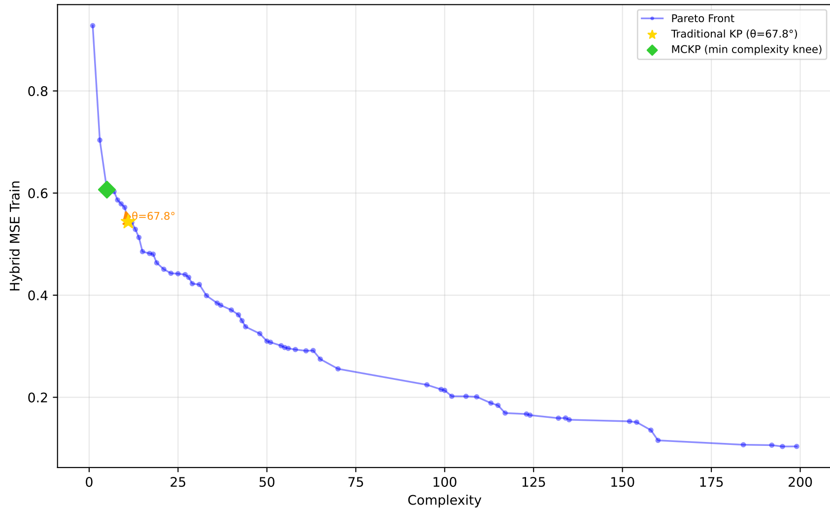
678_visualizing_environmental - Run 14 - MVP - Hybrid MSE Train \lambda_1=0.40, \lambda_2=0.00, \lambda_3=0.00 | Difficulty: 0.25 | Method: mckp
