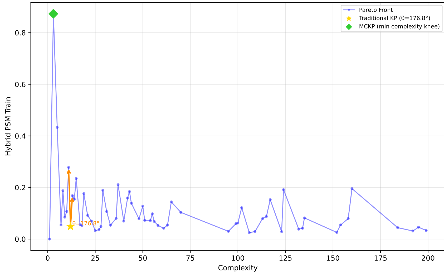
678_visualizing_environmental - Run 14 - MVP - Hybrid PSM Train \lambda_1=0.40, \lambda_2=0.00, \lambda_3=0.00 | Difficulty: 0.25 | Method: mckp
