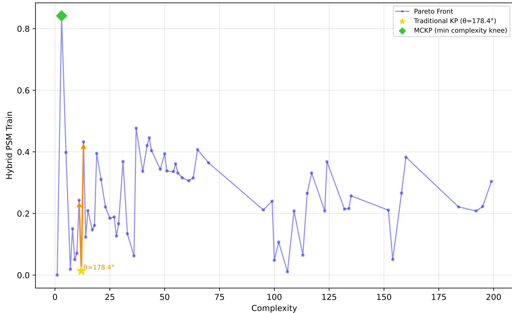
678_visualizing_environmental - Run 14 - SVP - Hybrid PSM Train \lambda_1=0.00, \lambda_2=0.10, \lambda_3=0.20 | Difficulty: 0.25 | Method: mckp
