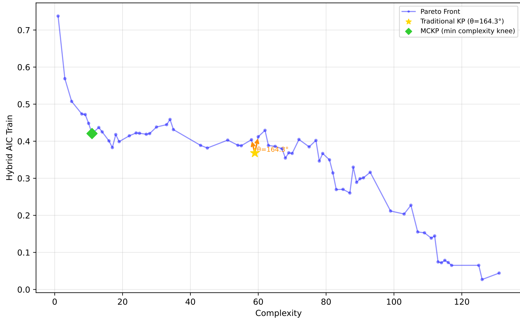
678_visualizing_environmental - Run 15 - MVP - Hybrid AIC Train \lambda_1=0.00, \lambda_2=0.00, \lambda_3=0.10 | Difficulty: 0.19 | Method: mckp
