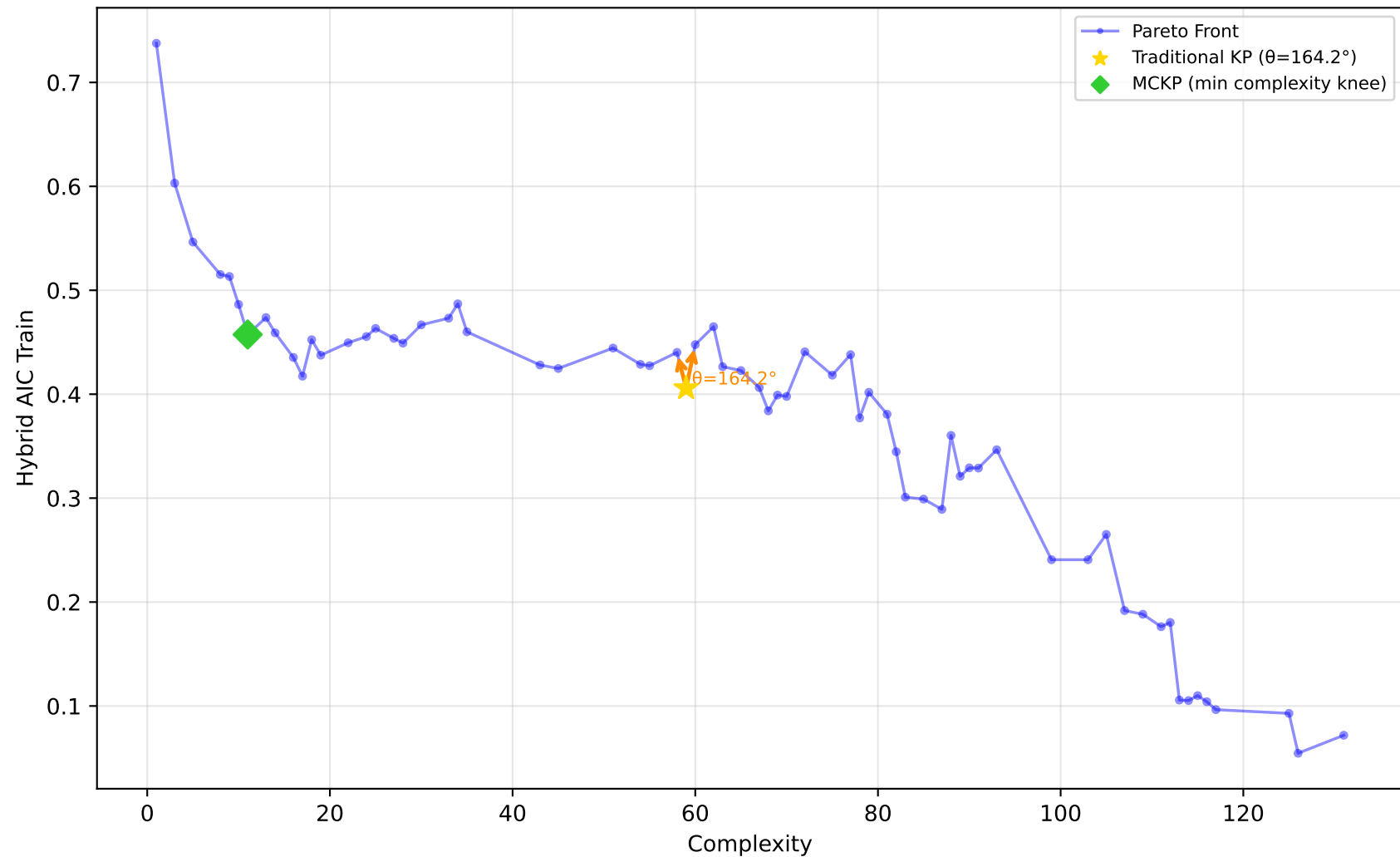
678_visualizing_environmental - Run 15 - MVP - Hybrid AIC Train \lambda_1=0.40 , \lambda_2=0.00 , \lambda_3=0.00 | Difficulty: 0.19 | Method: mckp
