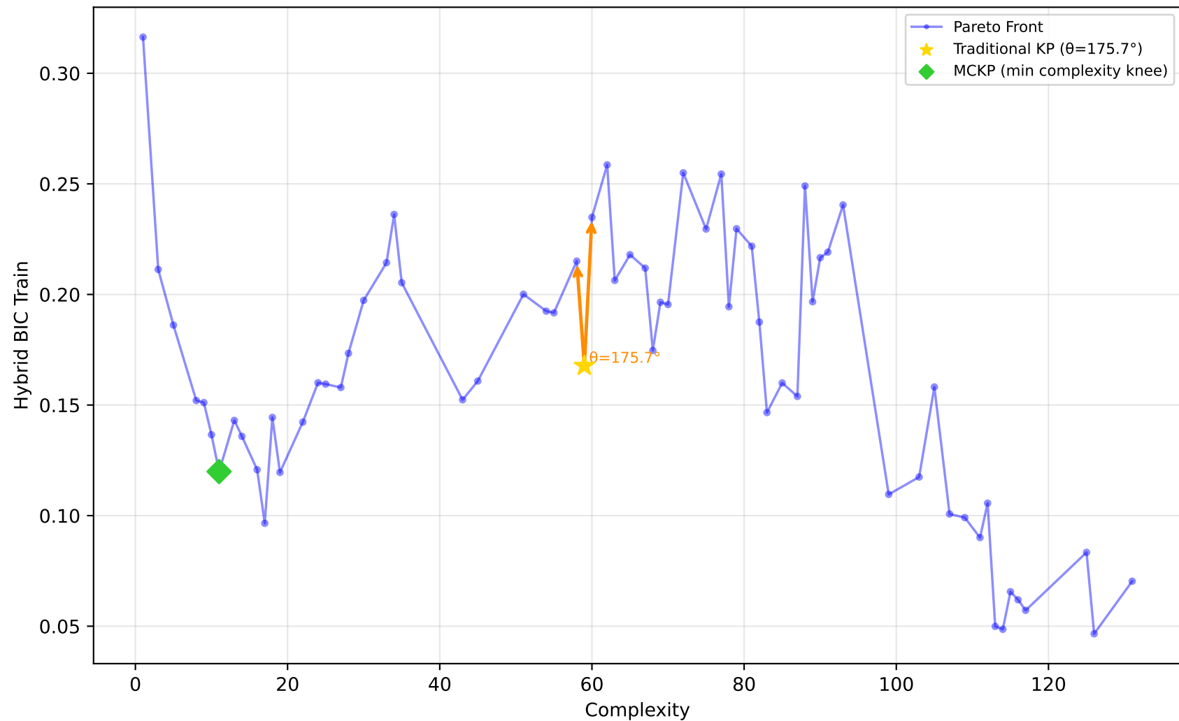
678_visualizing_environmental - Run 15 - MVP - Hybrid BIC Train \lambda_1=0.00, \lambda_2=0.00, \lambda_3=0.10 | Difficulty: 0.19 | Method: mckp
